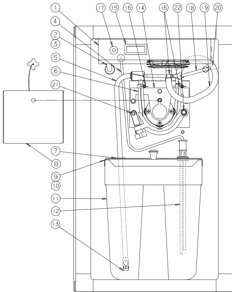
Figure 5 Cabinet Parts
