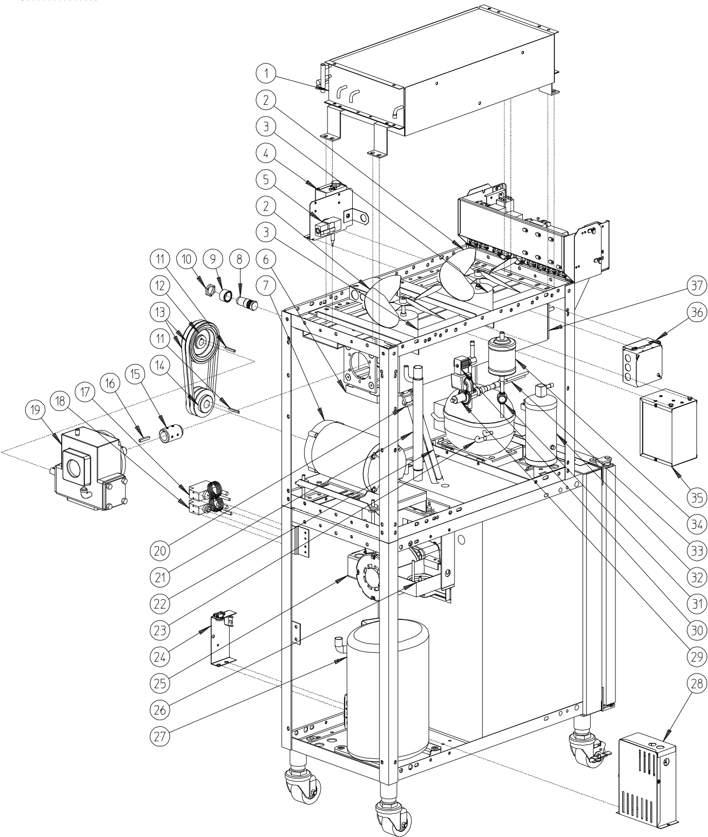
Figure 10 Rear/Side View Air Cooled (sheet 1 of 2)
