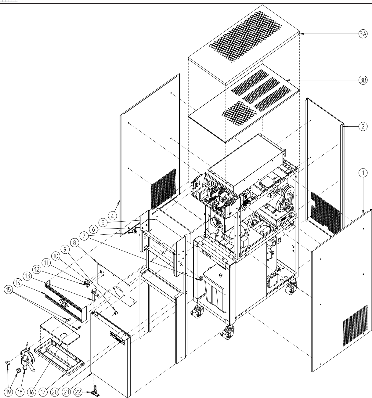
Figure 9 Panel Assembly (sheet 1 of 2)
