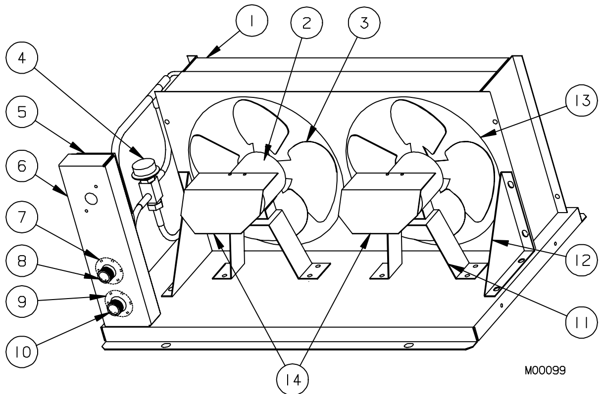
Figure 9 Air Cooled Remote Condenser Assembly
