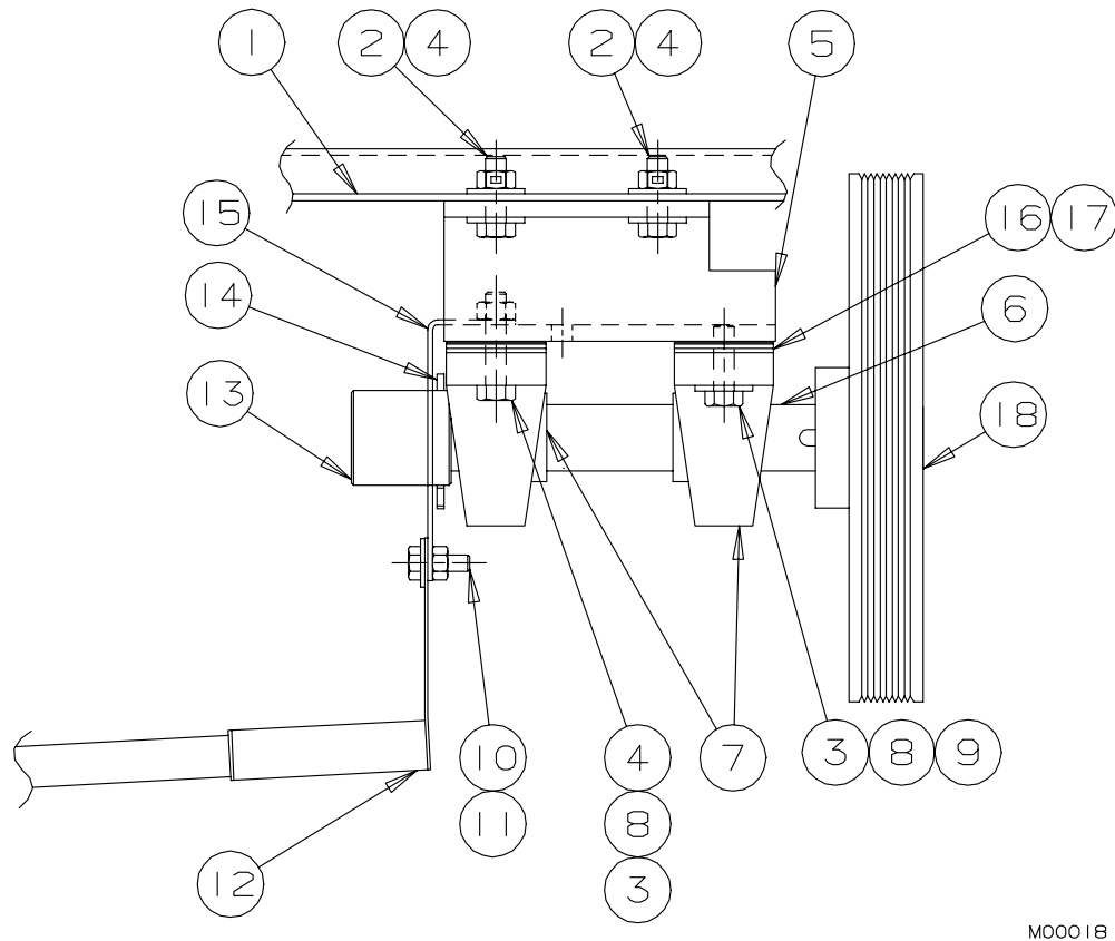
Figure 5 Drive Shaft and Bearing Assembly
