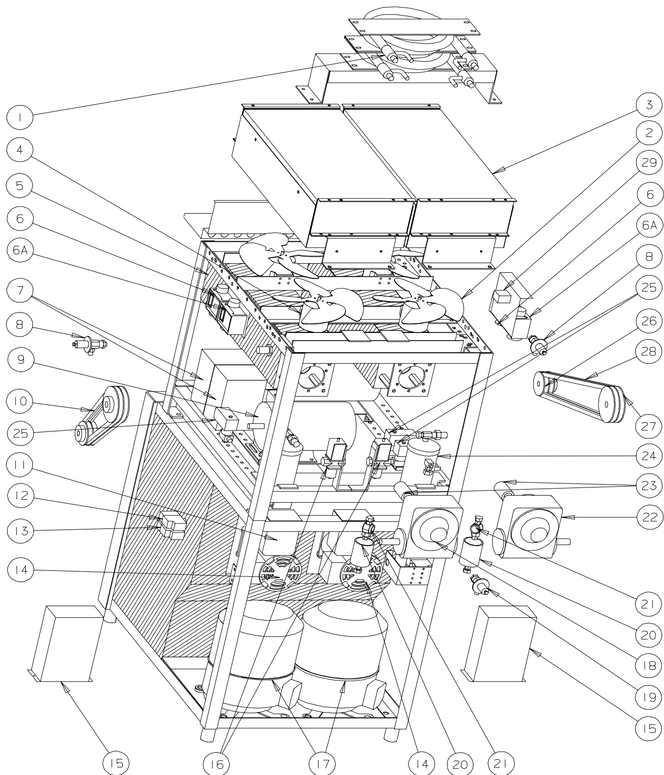
Figure 9 30CMT Side/Back View (sheet 1 of 2)
