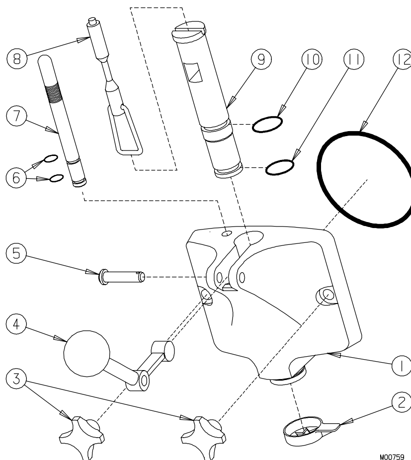
Figure 1 Head Assembly
