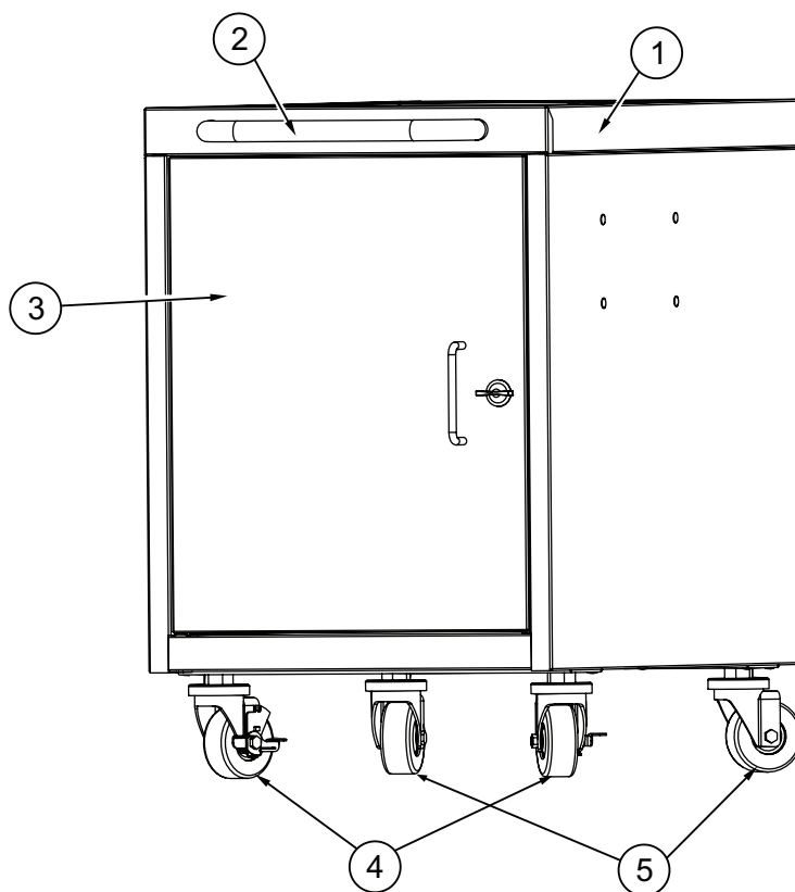
Figure 7 Cabinet Assembly
