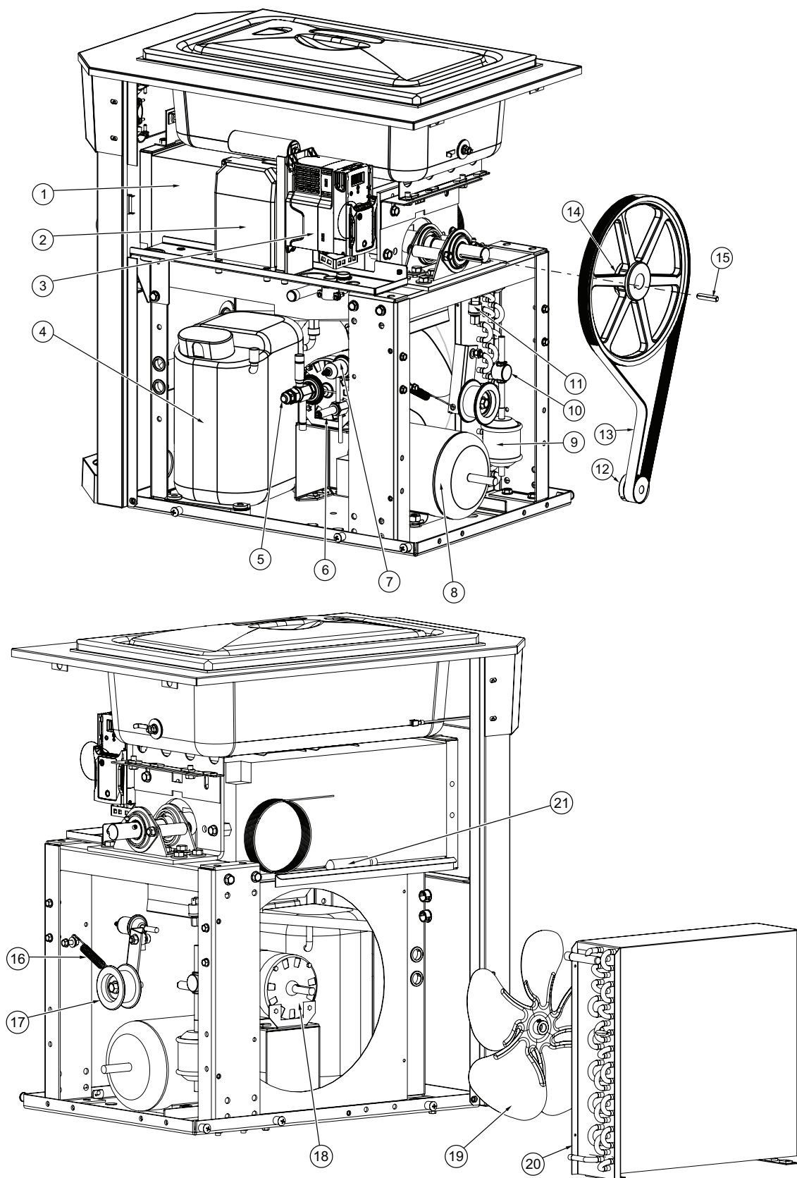
Figure 4 Assembly View
