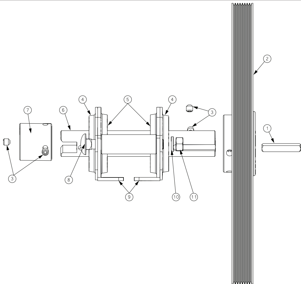
Figure 6 Drive Shaft and Bearing Assembly
