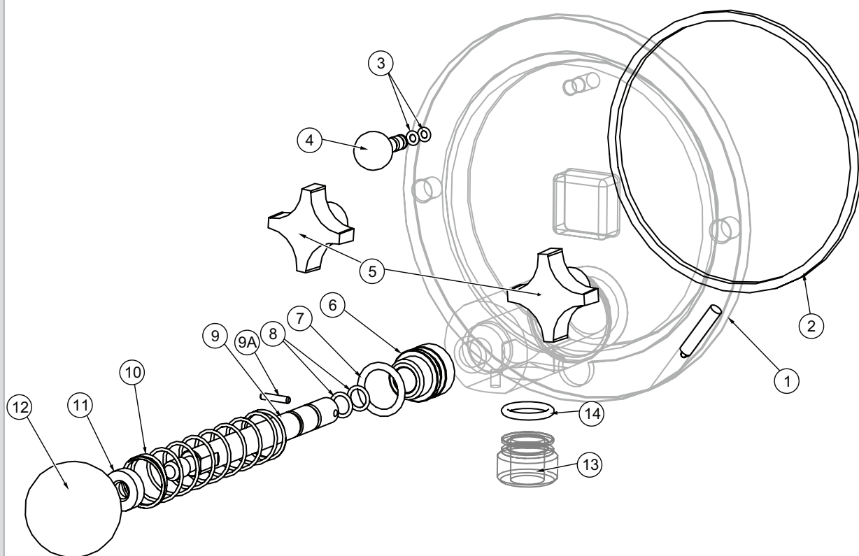
Figure 1 Pull Valve Door Assembly
