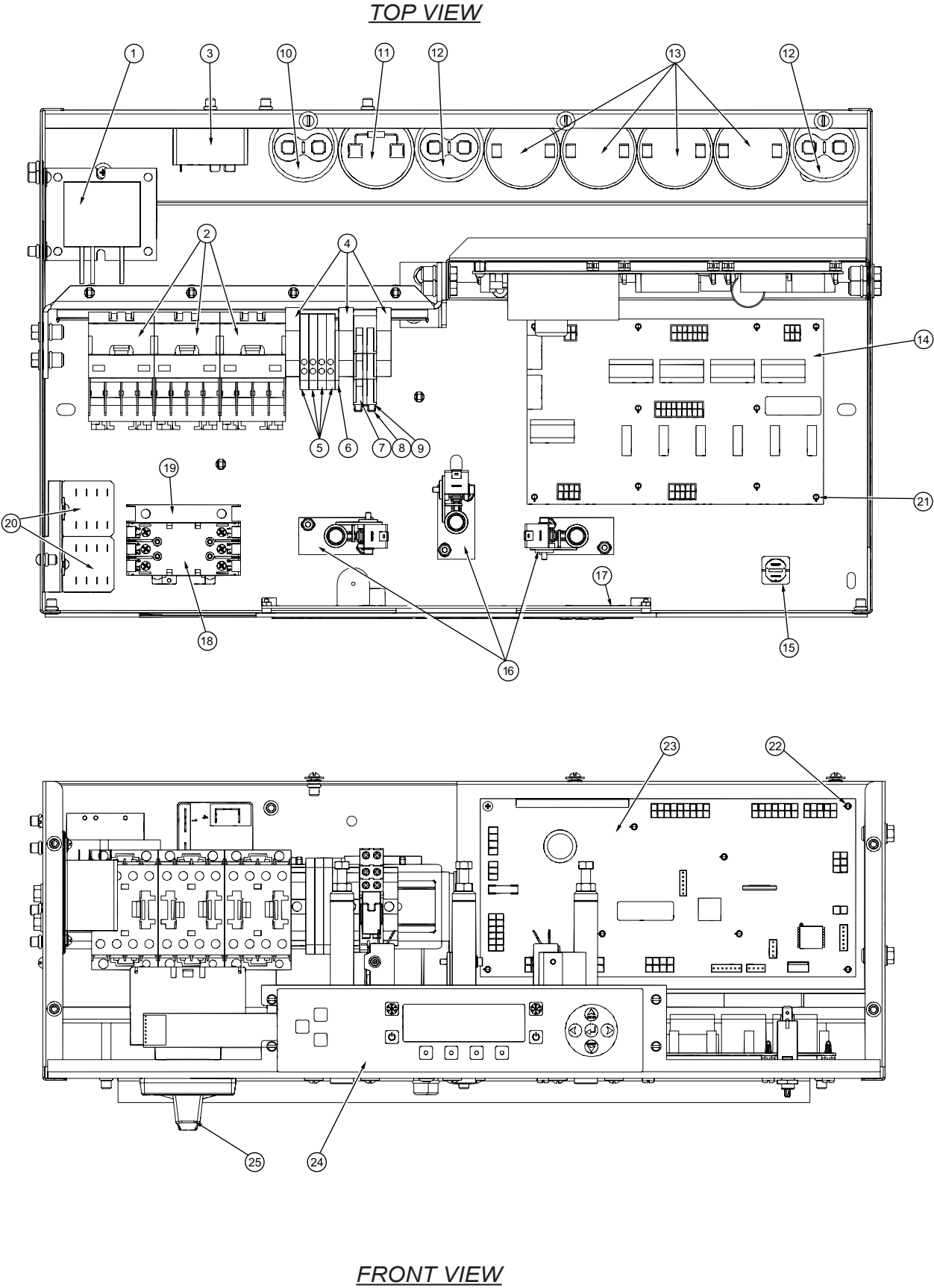
Figure 8 Switch Box (sheet 1 of 2)
