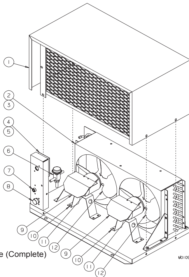
Figure 13 Air Cooled Remote Condenser
