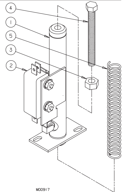
Figure 7 Capacitor & Relay Box (1 Ph. Only)
