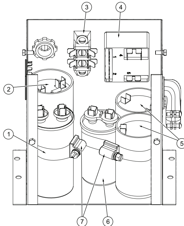
Figure 7 Capacitor & Relay Box (1 Ph. Only)
