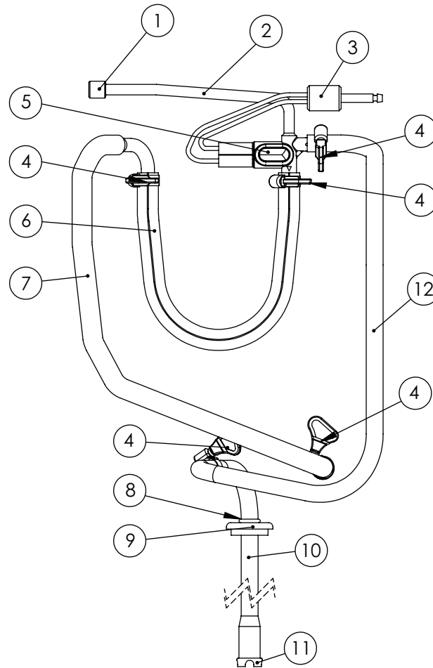
Figure 3 MTS—RMT Hose Assembly
