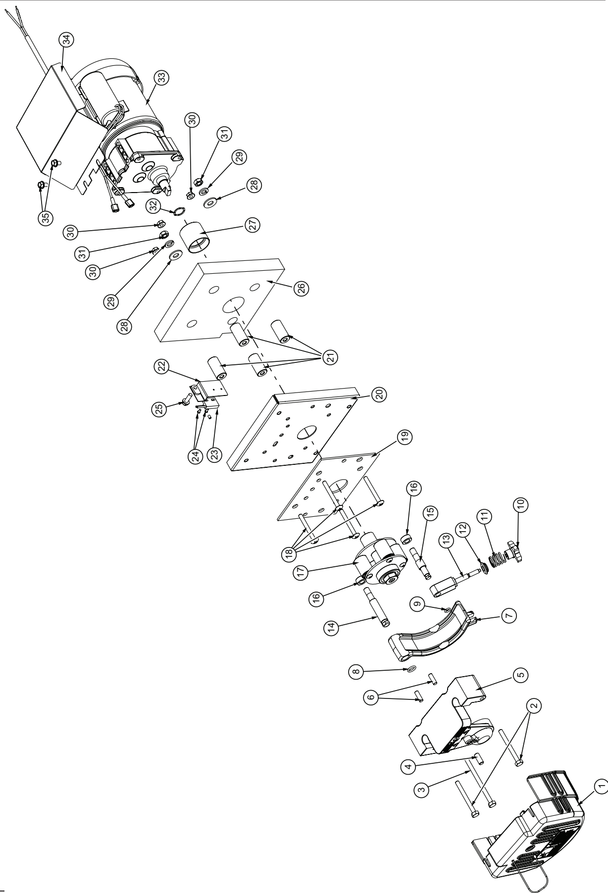
Figure 4 Mix Transfer System RMT 1Ph. (Sheet 1 of 2)
