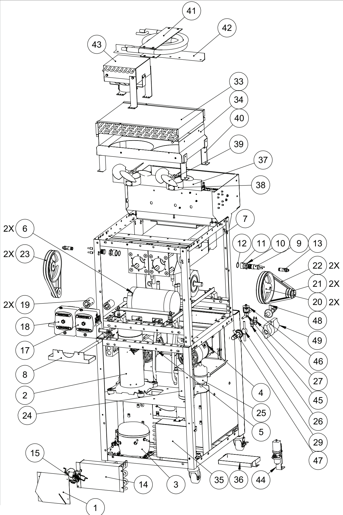
Figure 11 Side/Back View (Breakdown)
