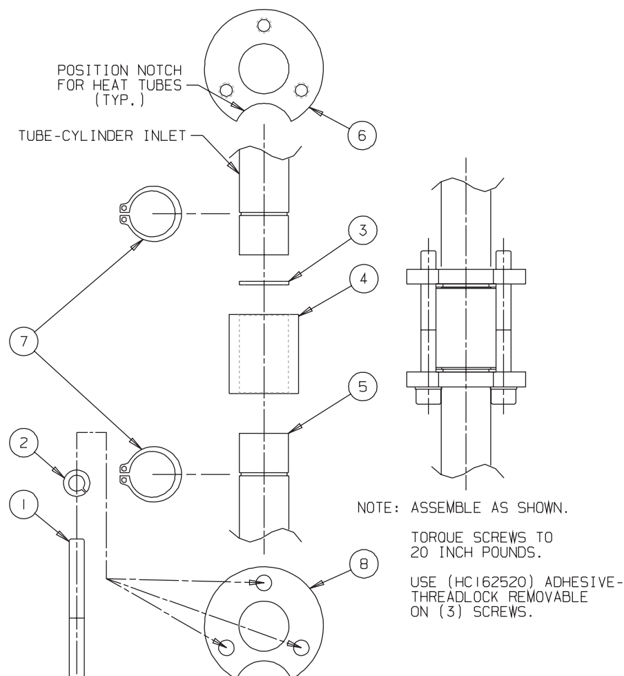
Figure 12 Mix Feed Seal Assembly
