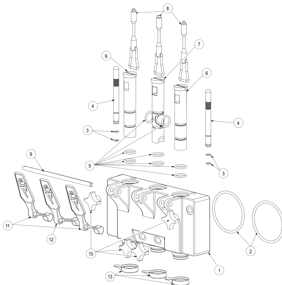
Figure 1 Head Assembly
