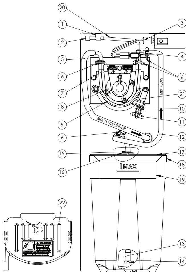
Figure 5 Cabinet Parts
