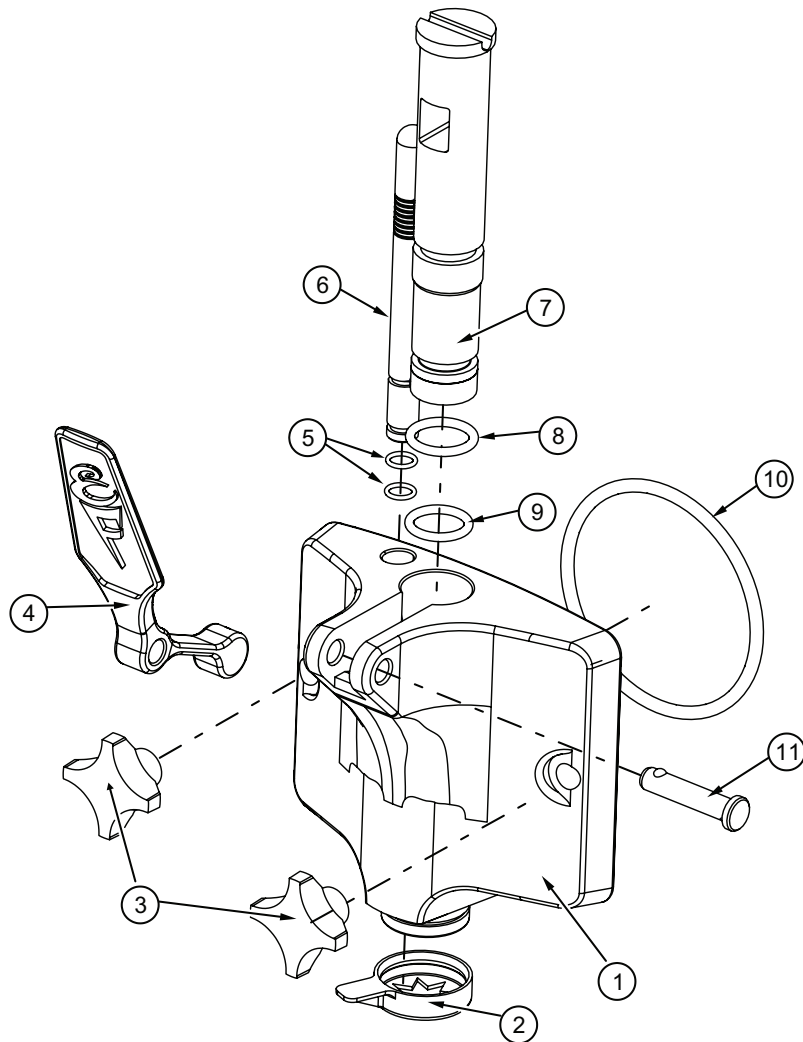
Figure 1 Soft Serve Head Assembly
