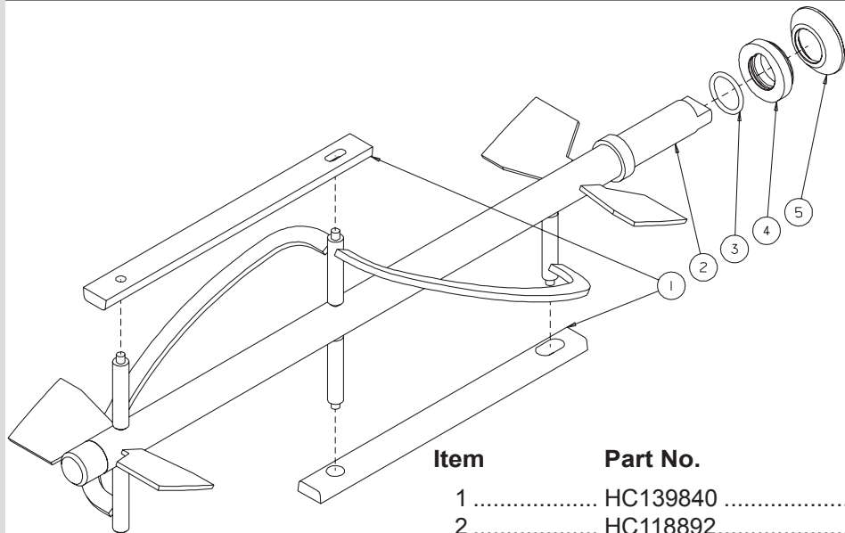
Figure 4 Shake Beater Shaft Assembly
