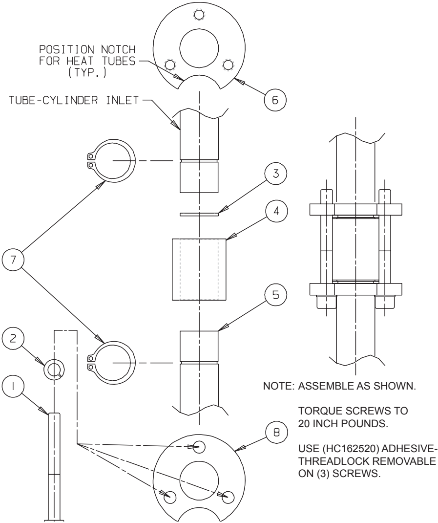
Figure 17 Mix Feed Seal Assembly
