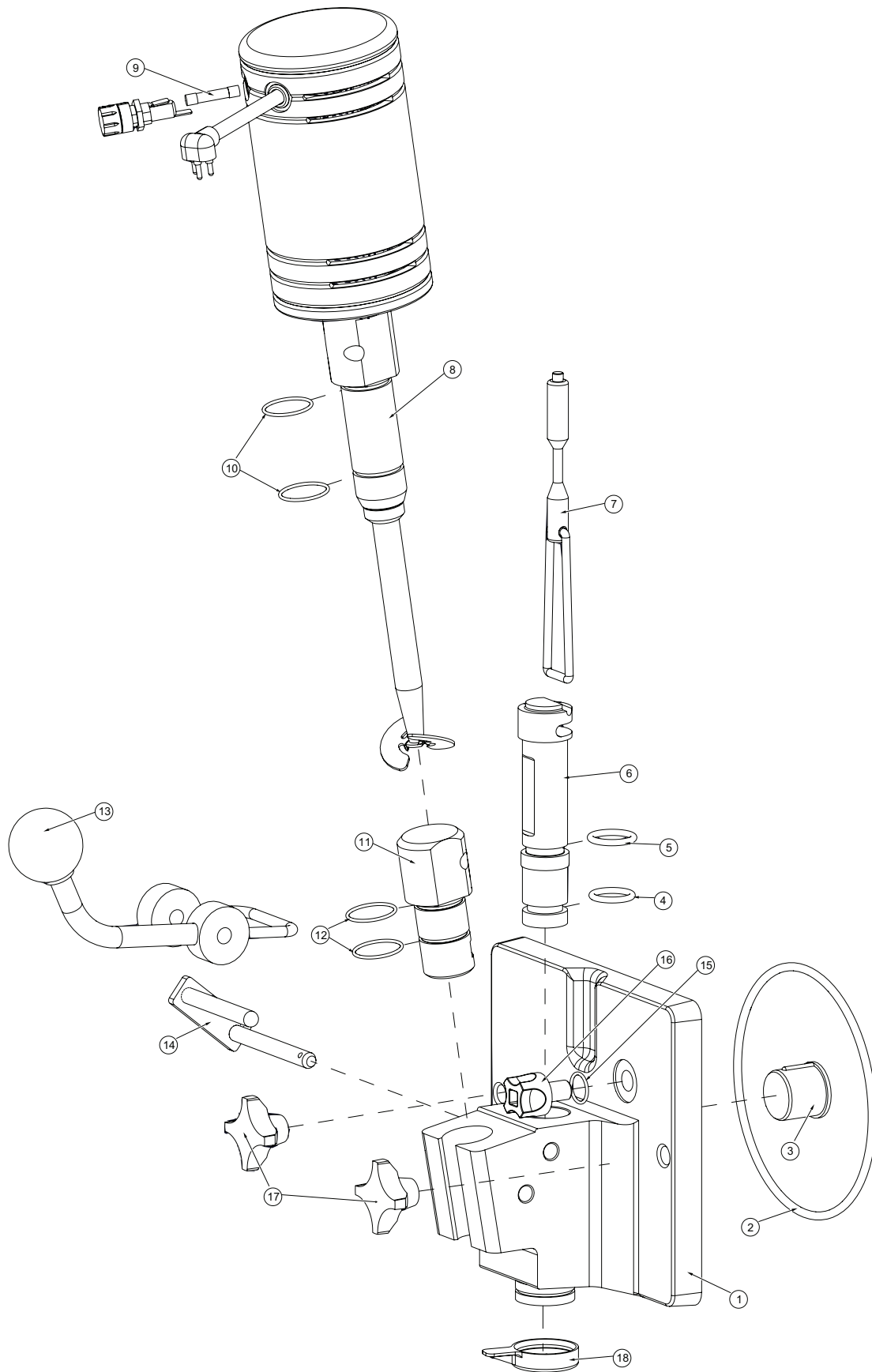
Figure 2 Shake Head Assembly (sheet 1 of 2)
