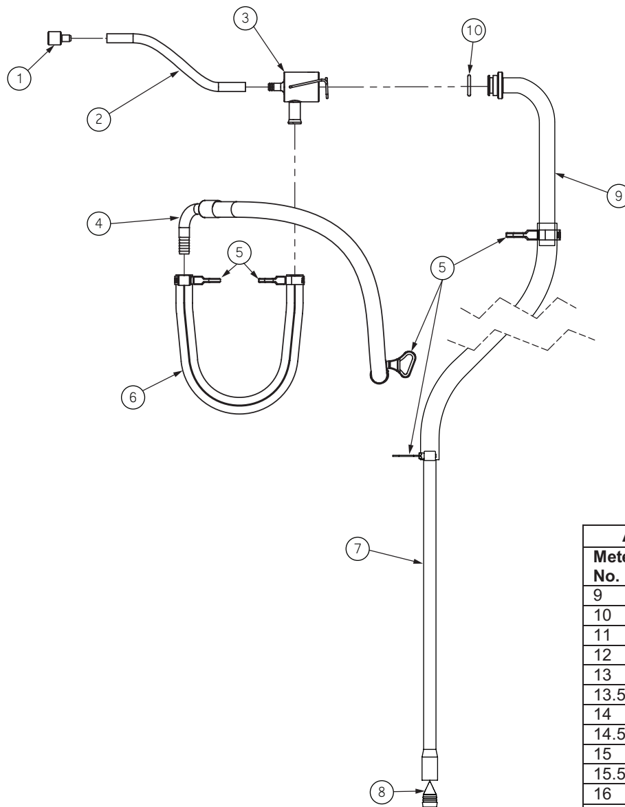
Figure 5 MTS—RMT Hose Assembly
