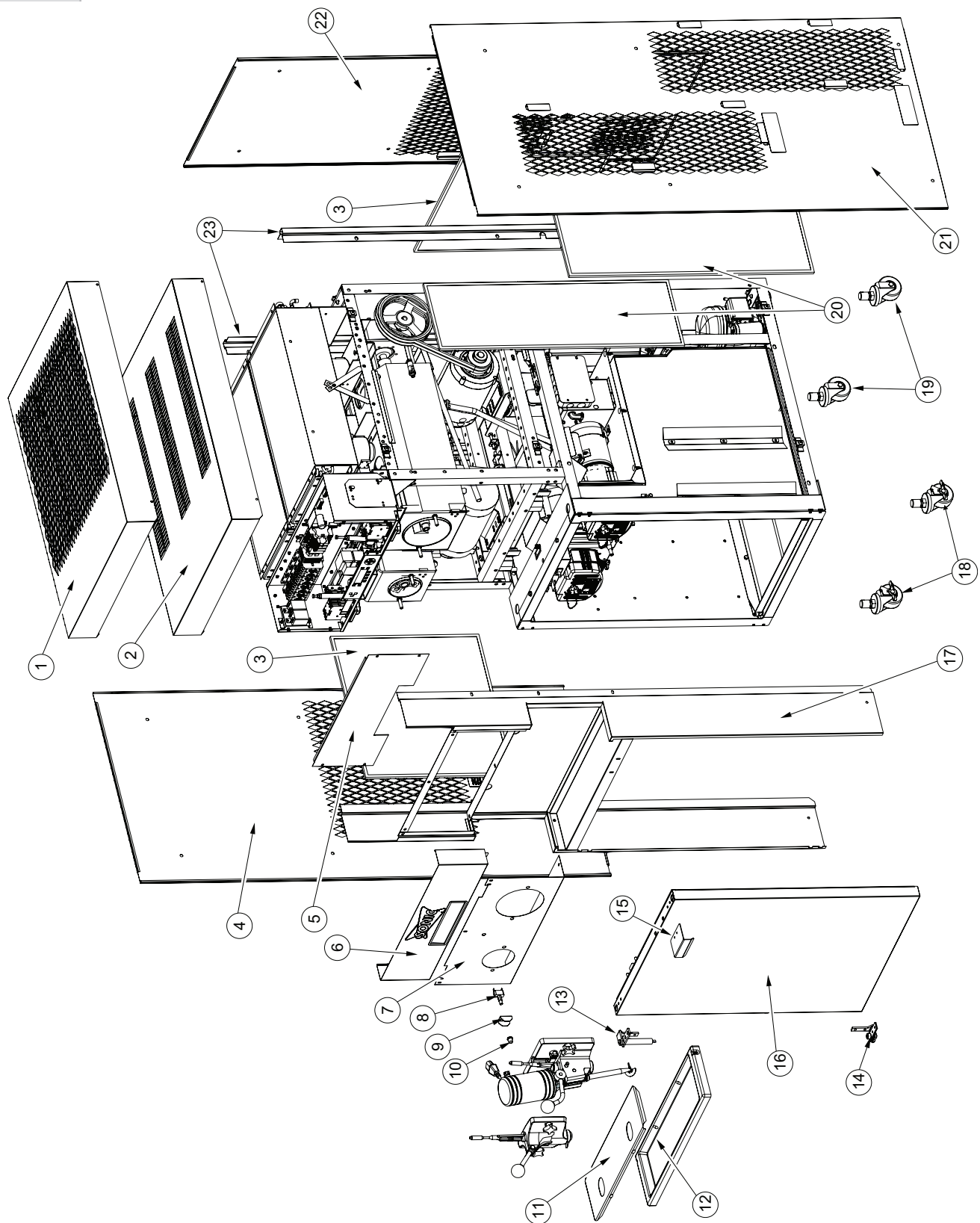
Figure 14 Panels (Sheet 1 of 2)
