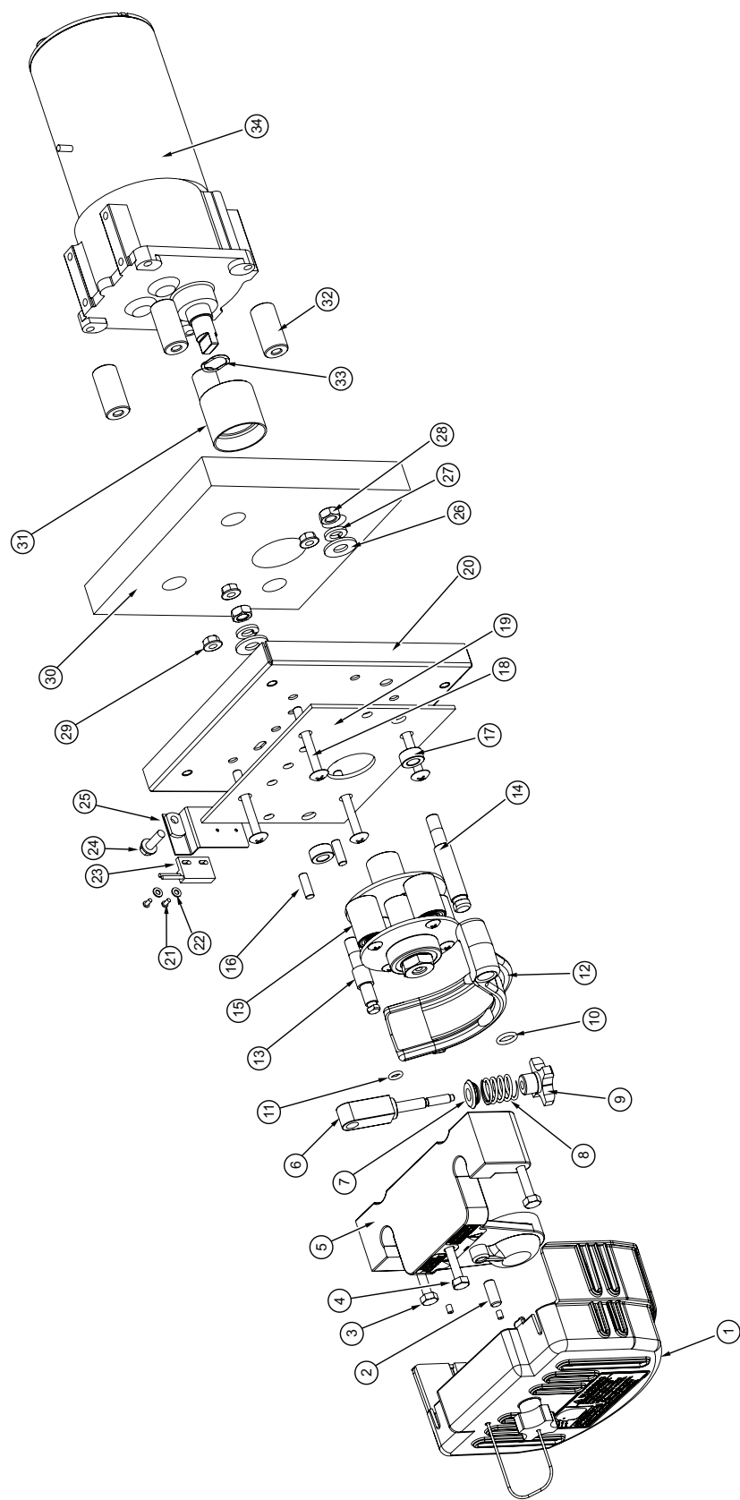
Figure 8 Mix Transfer System RMT 3Ph. (Sheet 1 of 2)
