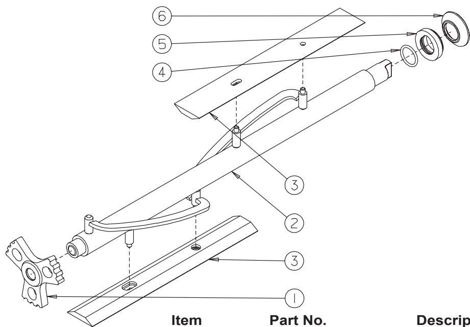
Figure 3 Soft Serve Beater Shaft Assembly
