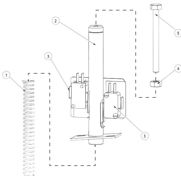
Figure 12 Switch Assembly - SH Side
