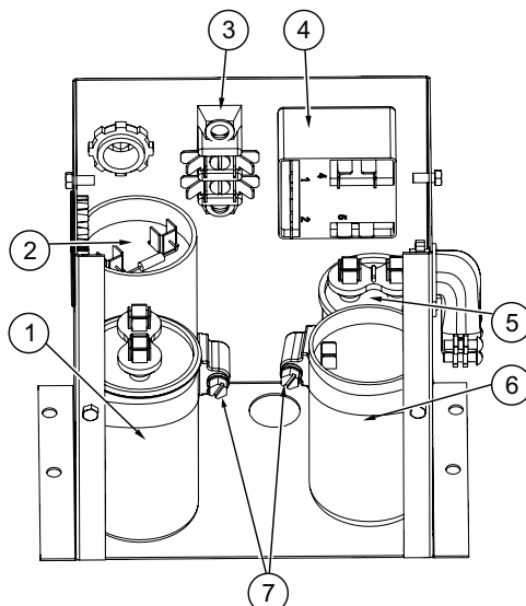
Figure 11 Capacitor & Relay Box 1Ph. SH Side
