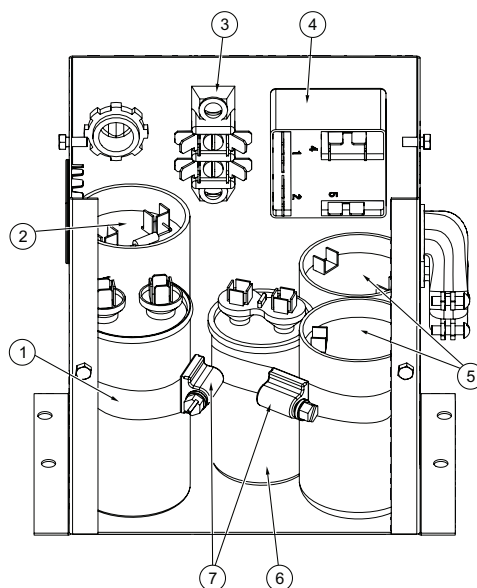
Figure 10 Capacitor & Relay Box 1Ph. SS Side
