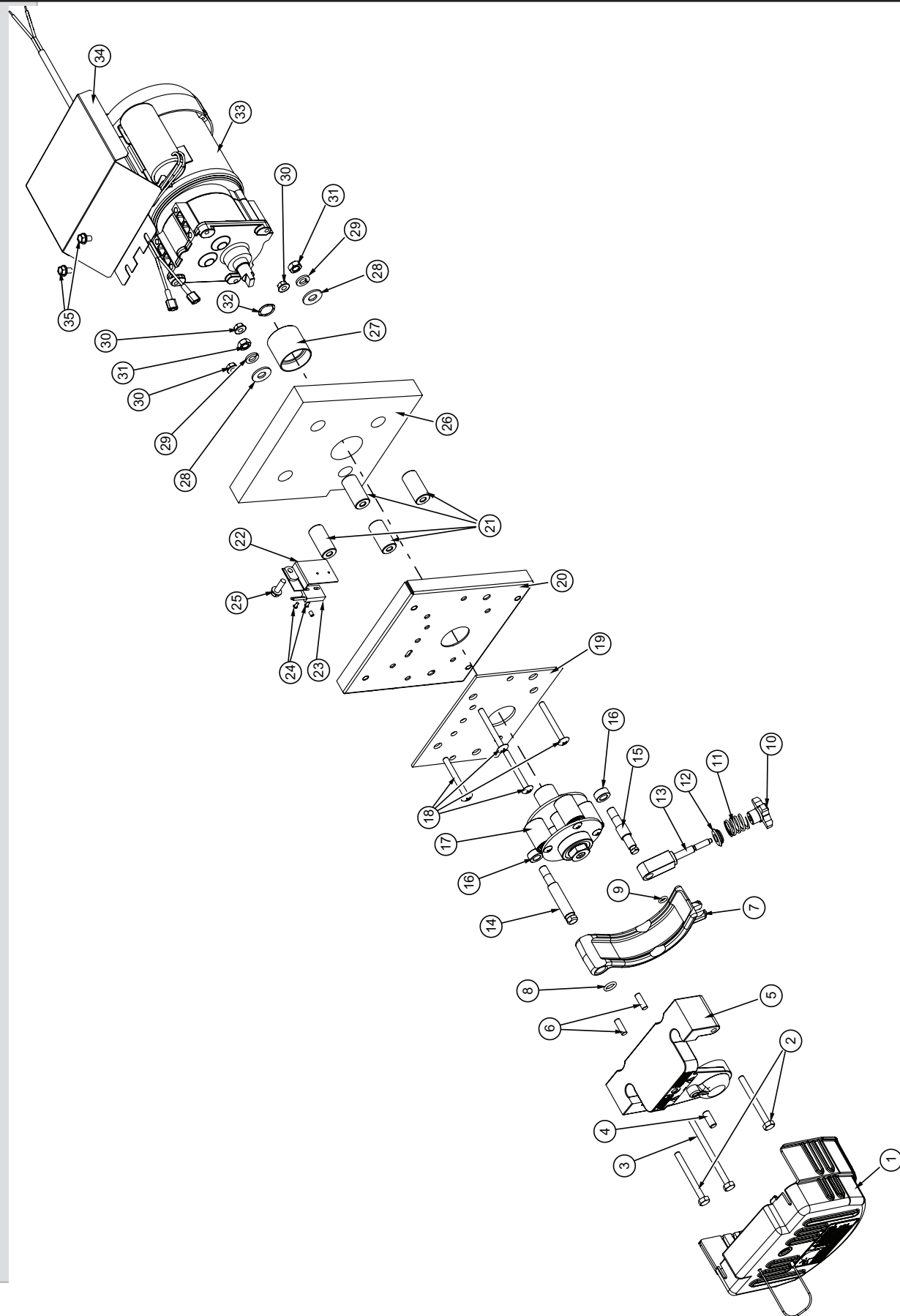
Figure 7 Mix Transfer System RMT 1Ph. (sheet 1 of 2)
