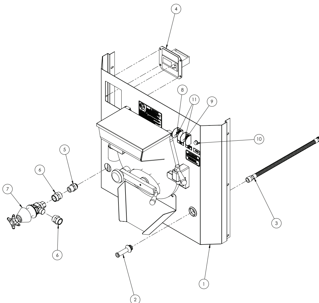
Figure 7 B12E Front Panel
