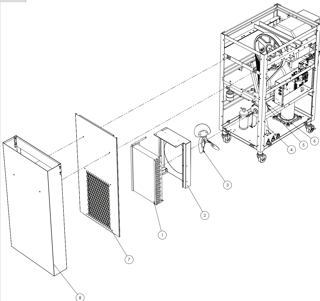
Figure 12 Rear Panel View
