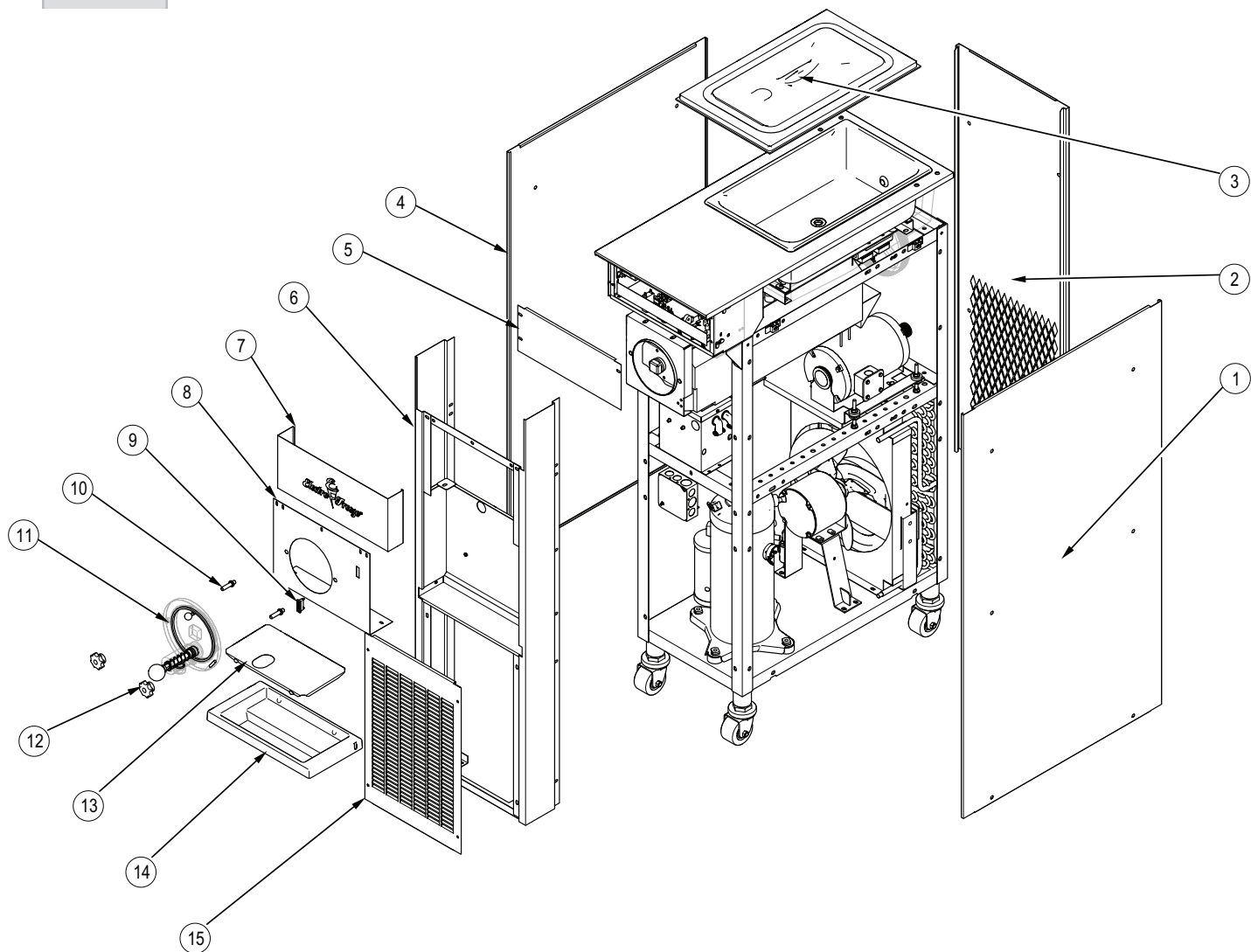
Figure 5 Panels - Air Cooled (Page 1 of 2)
