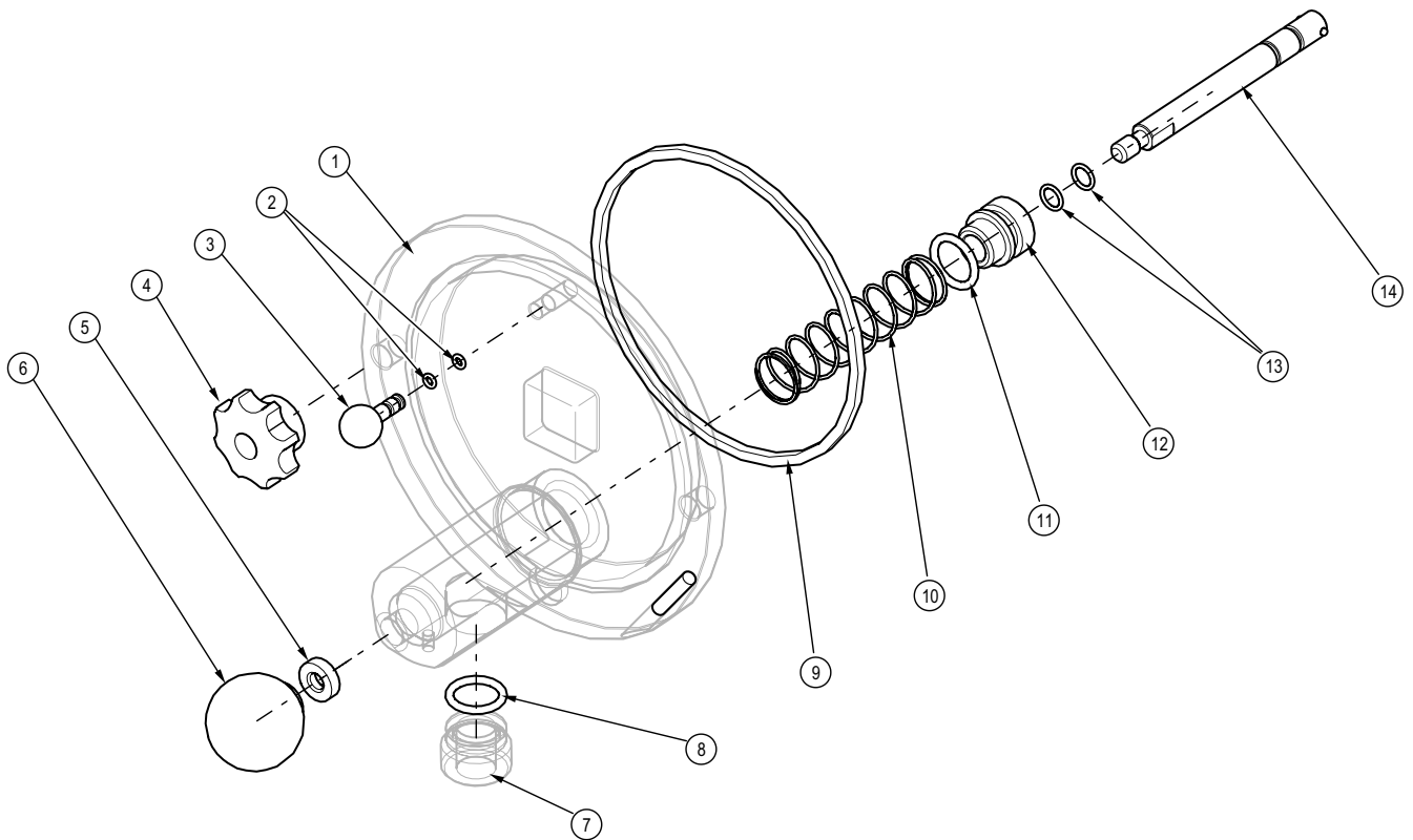
Figure 1 Door (Head) Assembly
