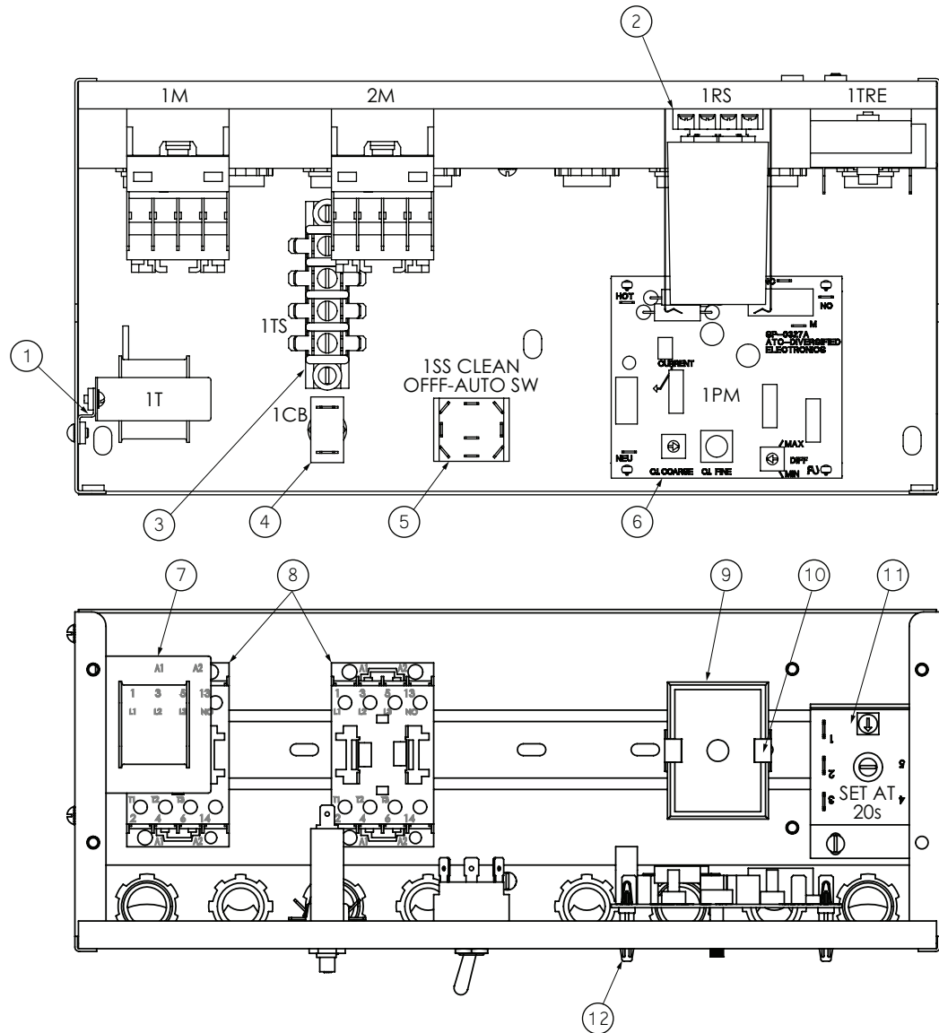
Figure 3 Electrical Box
