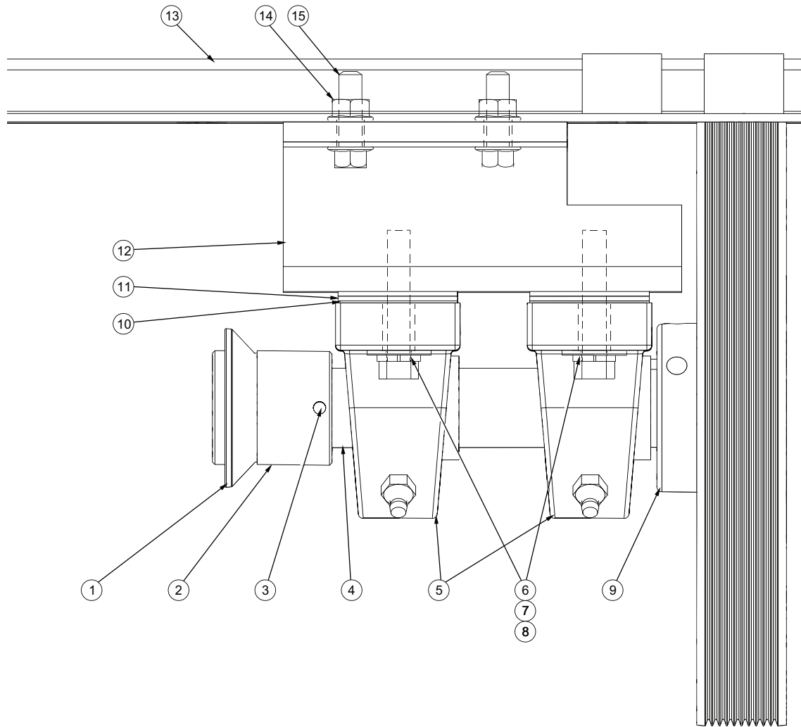
Figure 4 Drive Shaft and Bearing Assembly
