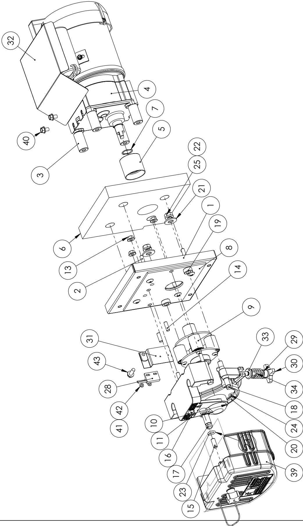
Figure 4 Mix Transfer System RMT (Sheet 1 of 2)
