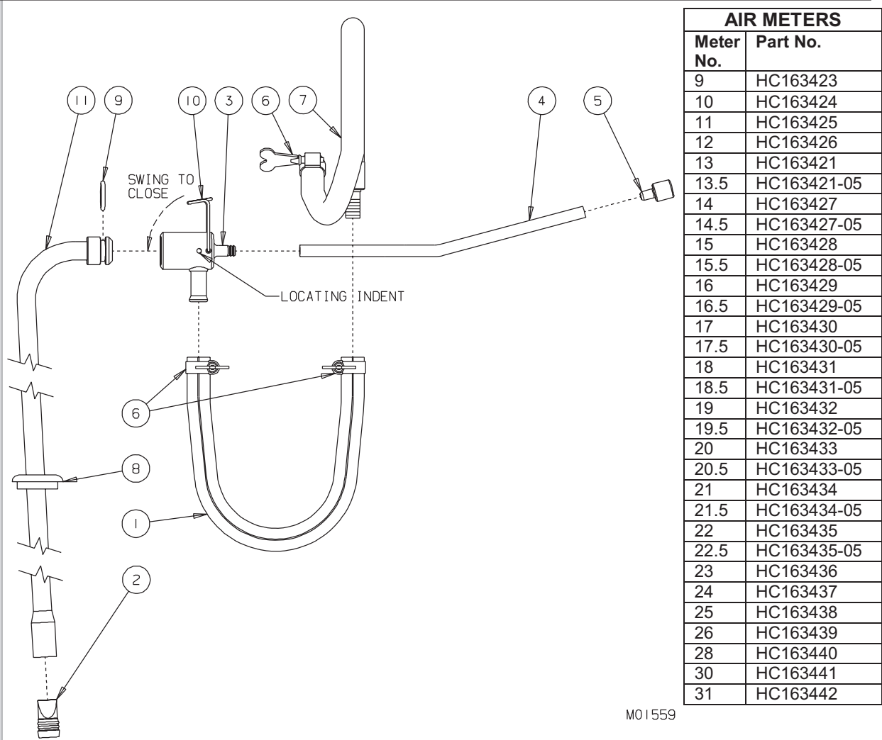
Figure 5 MTS - RMT Hose Assembly
