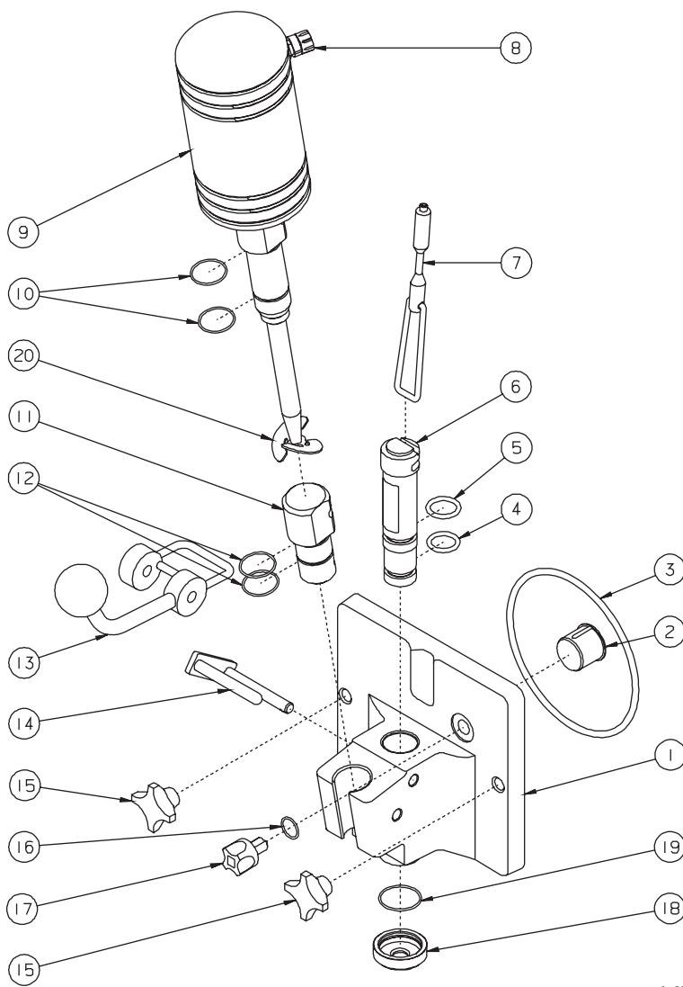
Figure 1 Head Assembly
