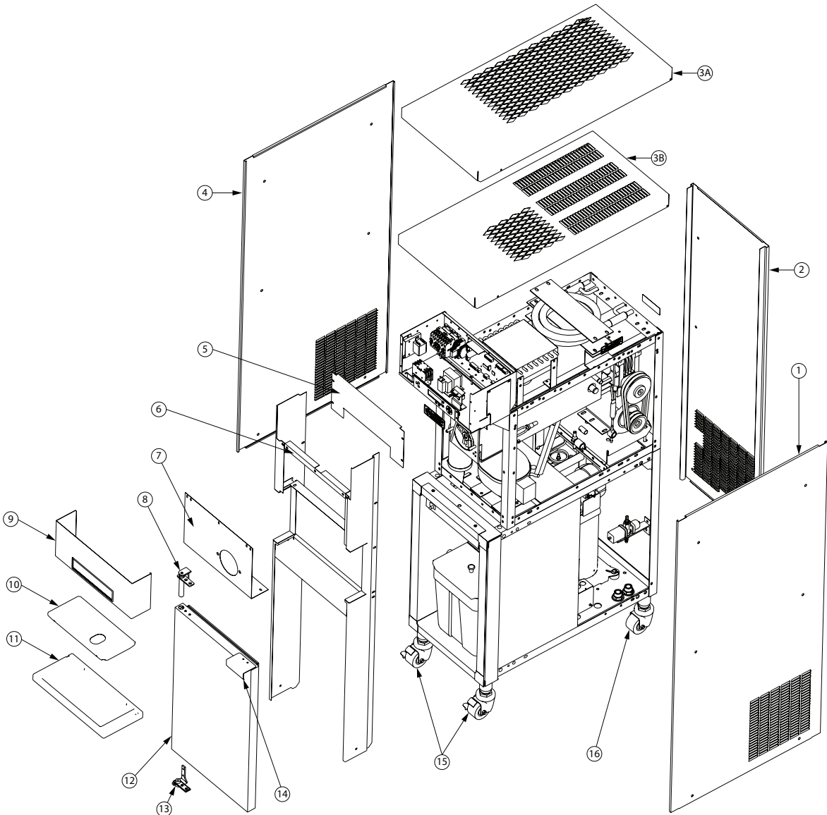
Figure 9 Panel Breakdown (Breakdown)
