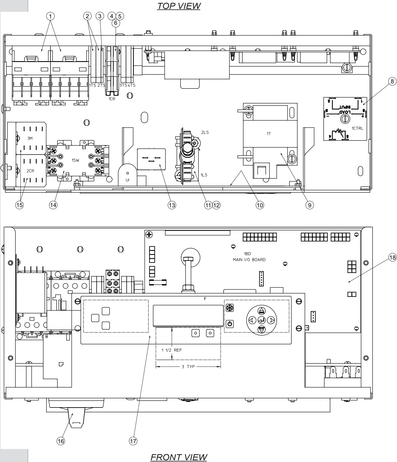
Figure 8 Switch Box (sheet 1 of 2)
