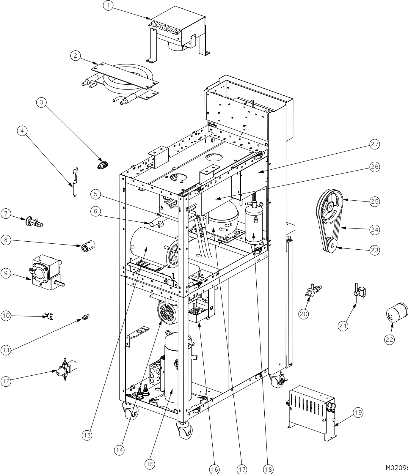
Figure 12 WC Side/Back View (Breakdown)
