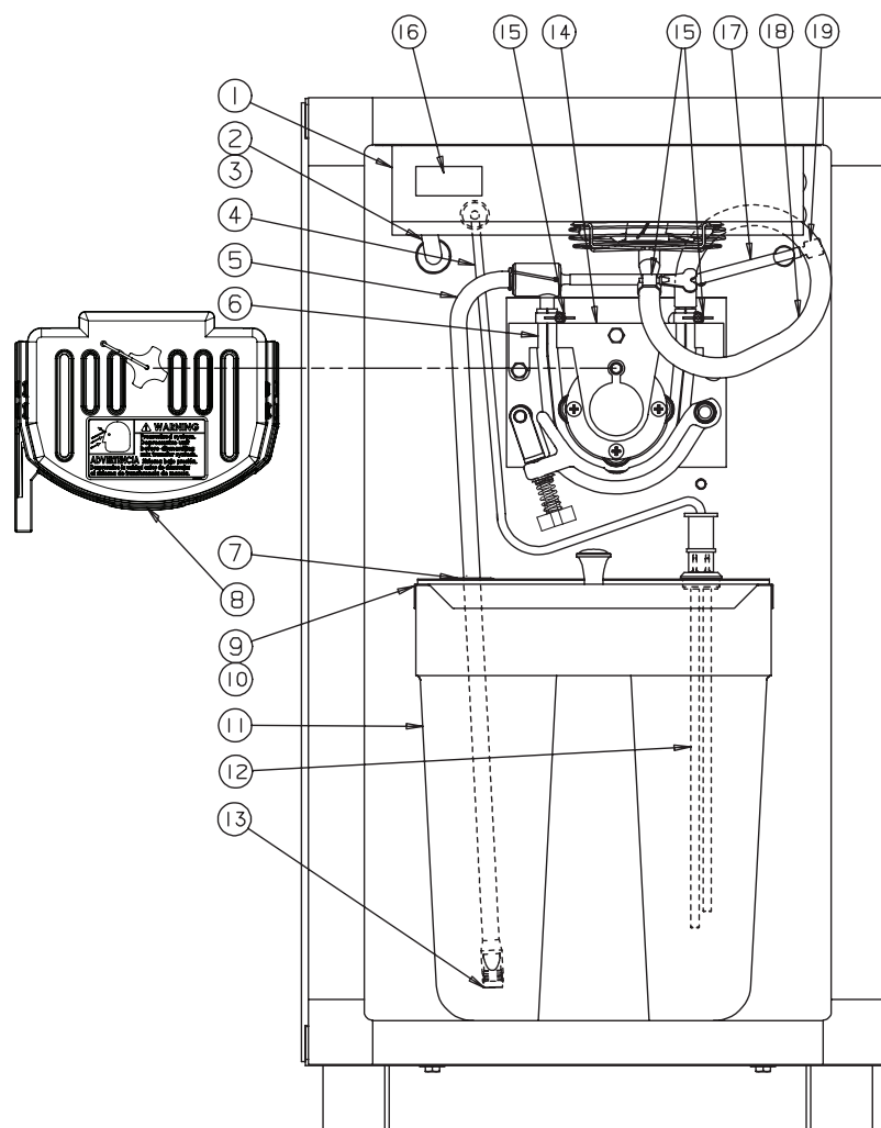
Figure 3 Cabinet Parts
