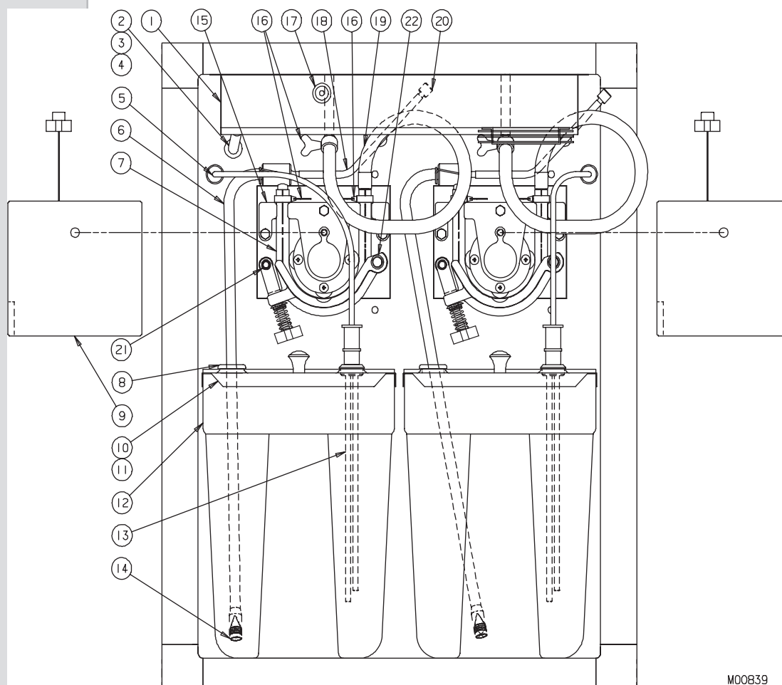
Figure 5 Cabinet Parts
