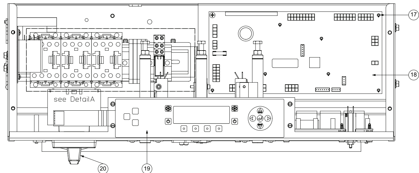
FRONT VIEW
