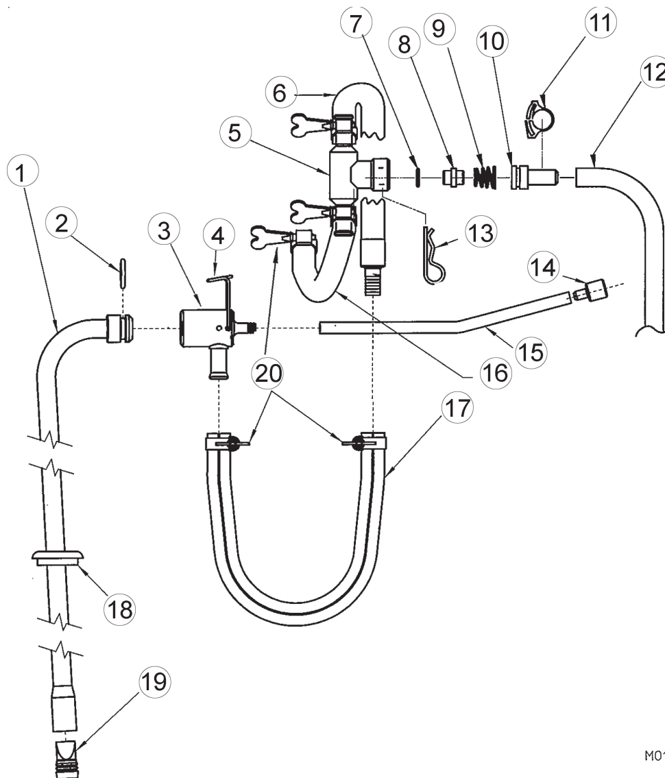
Figure 3 MTS—RMT Hose Assembly
