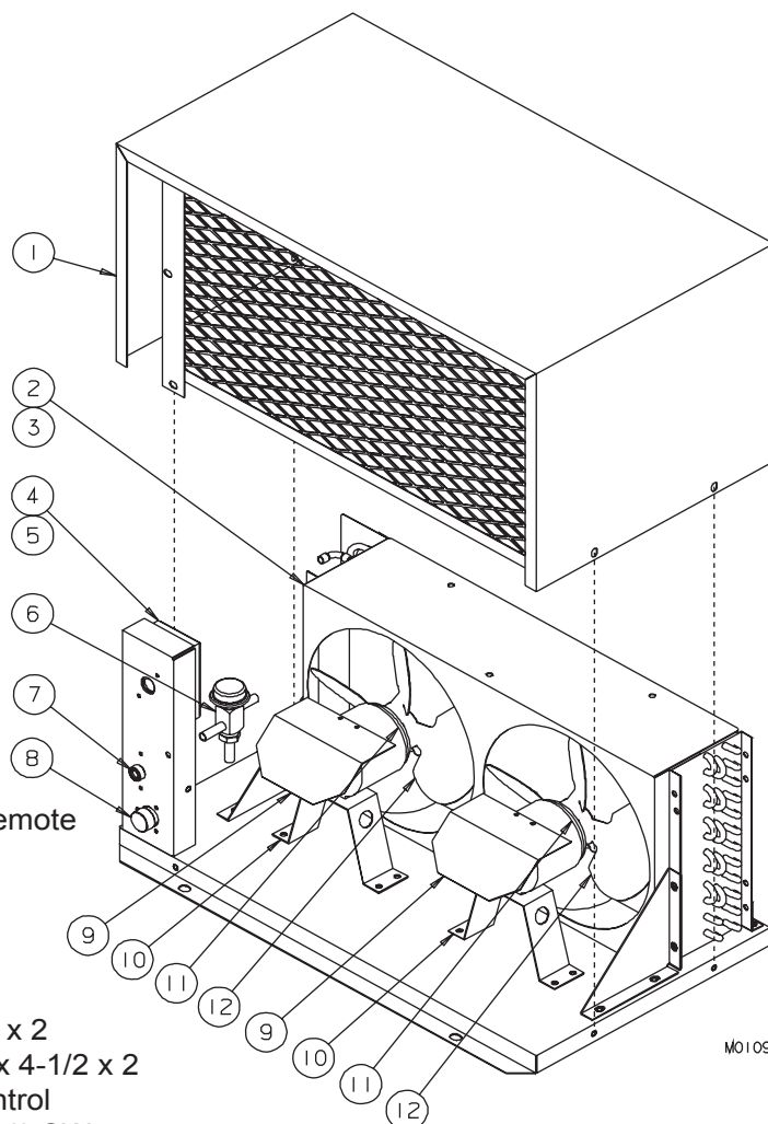
Figure 16 Air Cooled Remote Condenser
