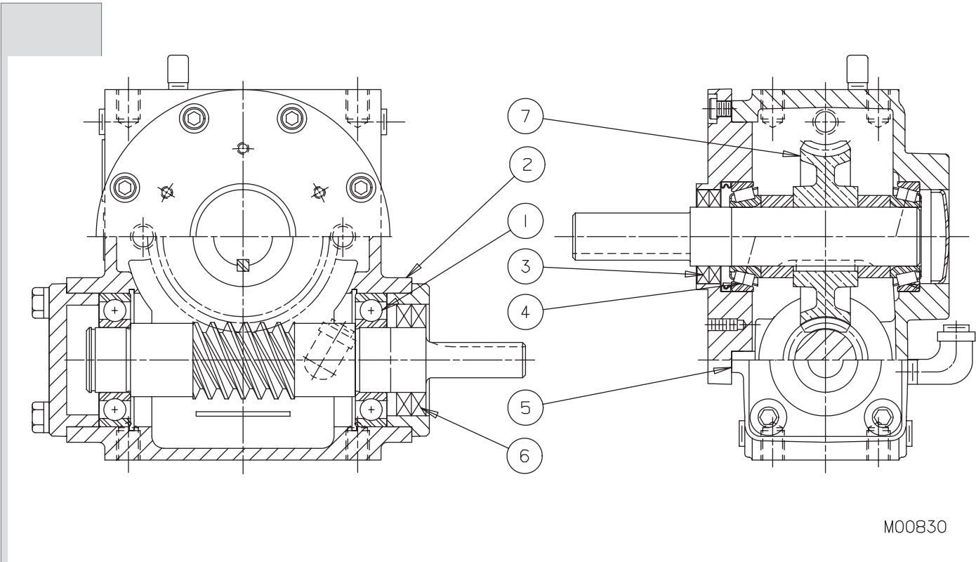
Figure 14 Gear Reducers
