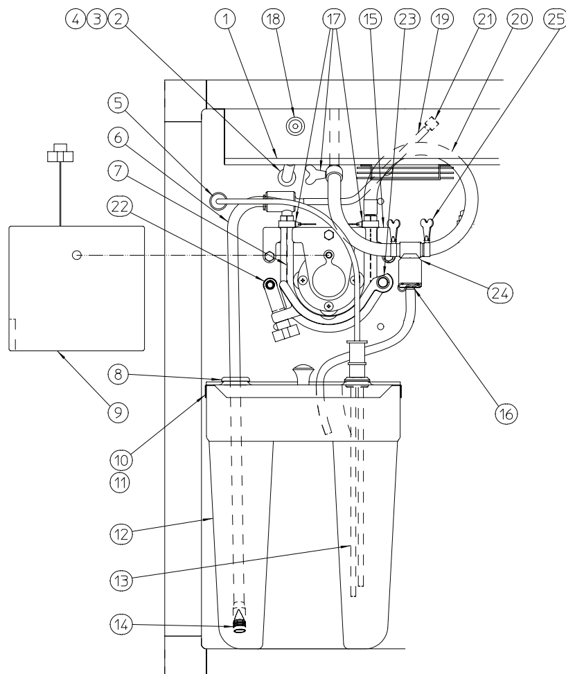
Figure 5 Cabinet Parts
