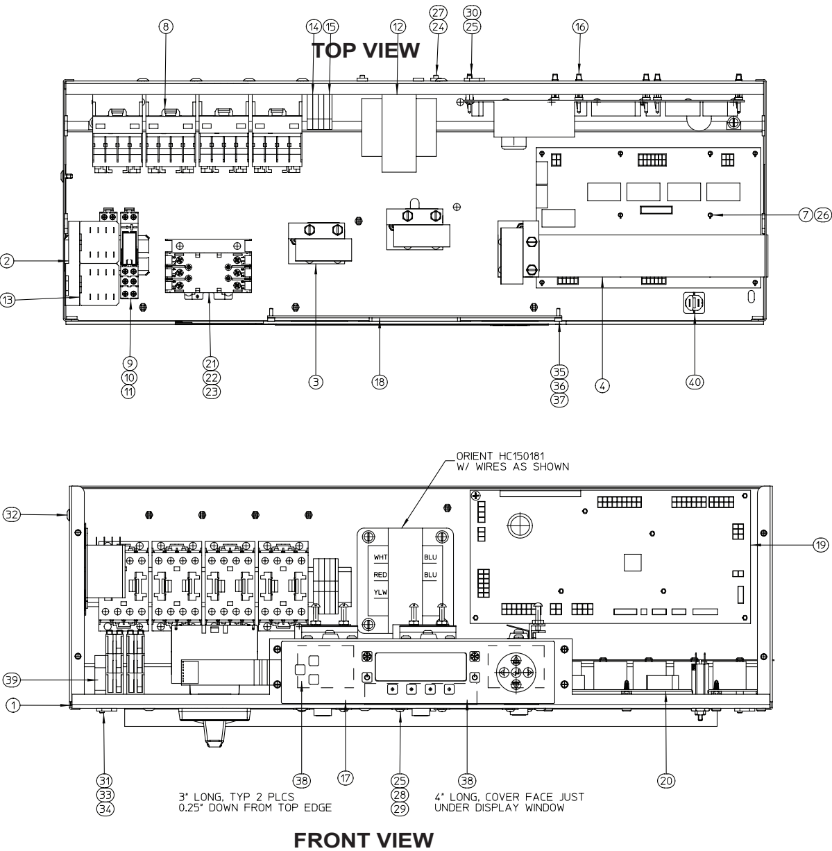
Figure 8 Switch Box (Breakdown)
