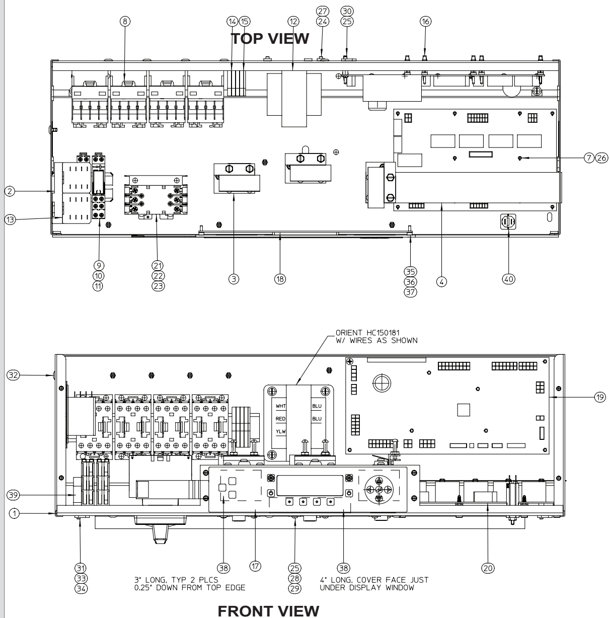
Figure 9 GEN-102 Switch Box (Breakdown)
