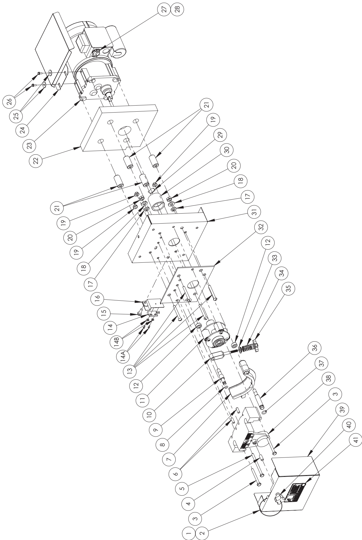
Figure 5 Mix Transfer System - RMT (sheet 1 of 2)
