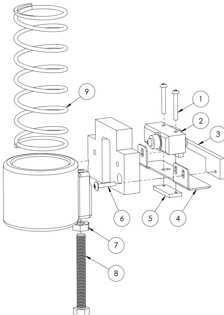
Figure 6 Switch Assembly
