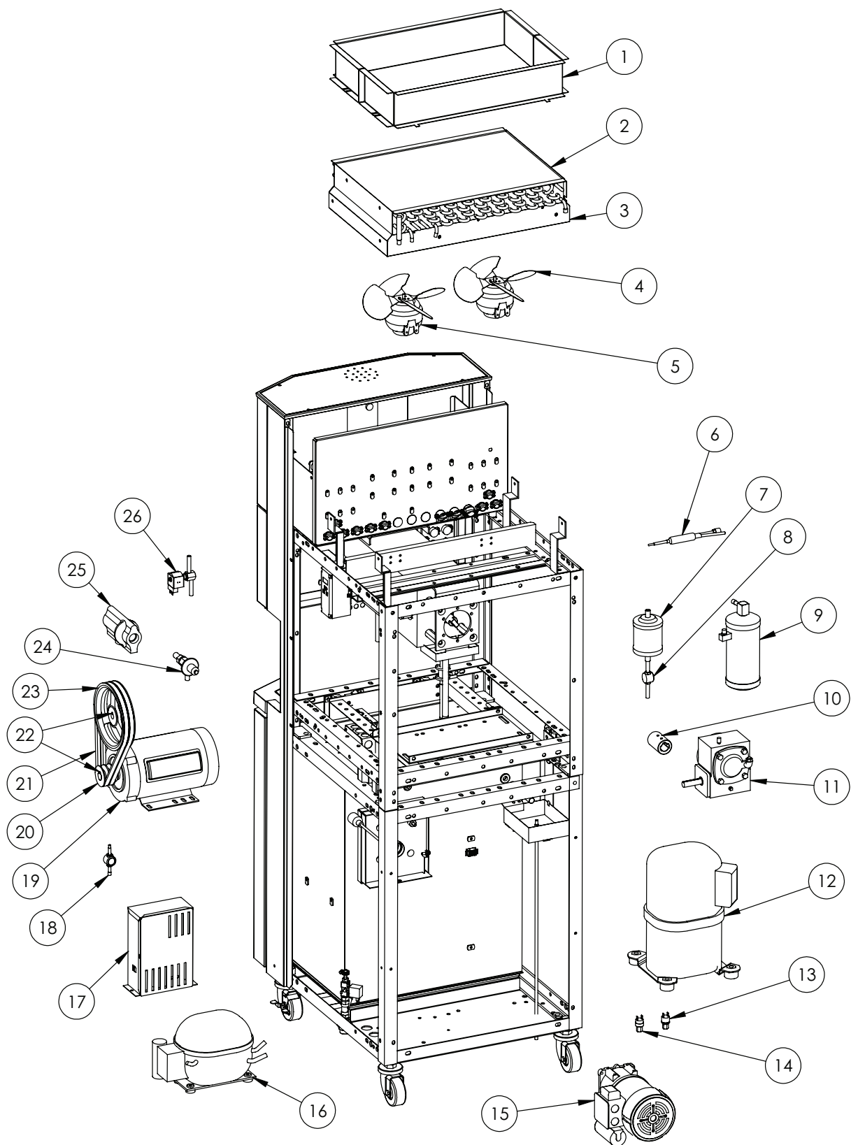
Figure 9 Air Cooled Assembly
