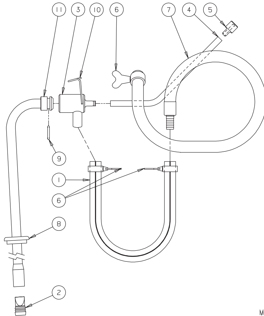
Figure 3 MTS Hose Assembly
