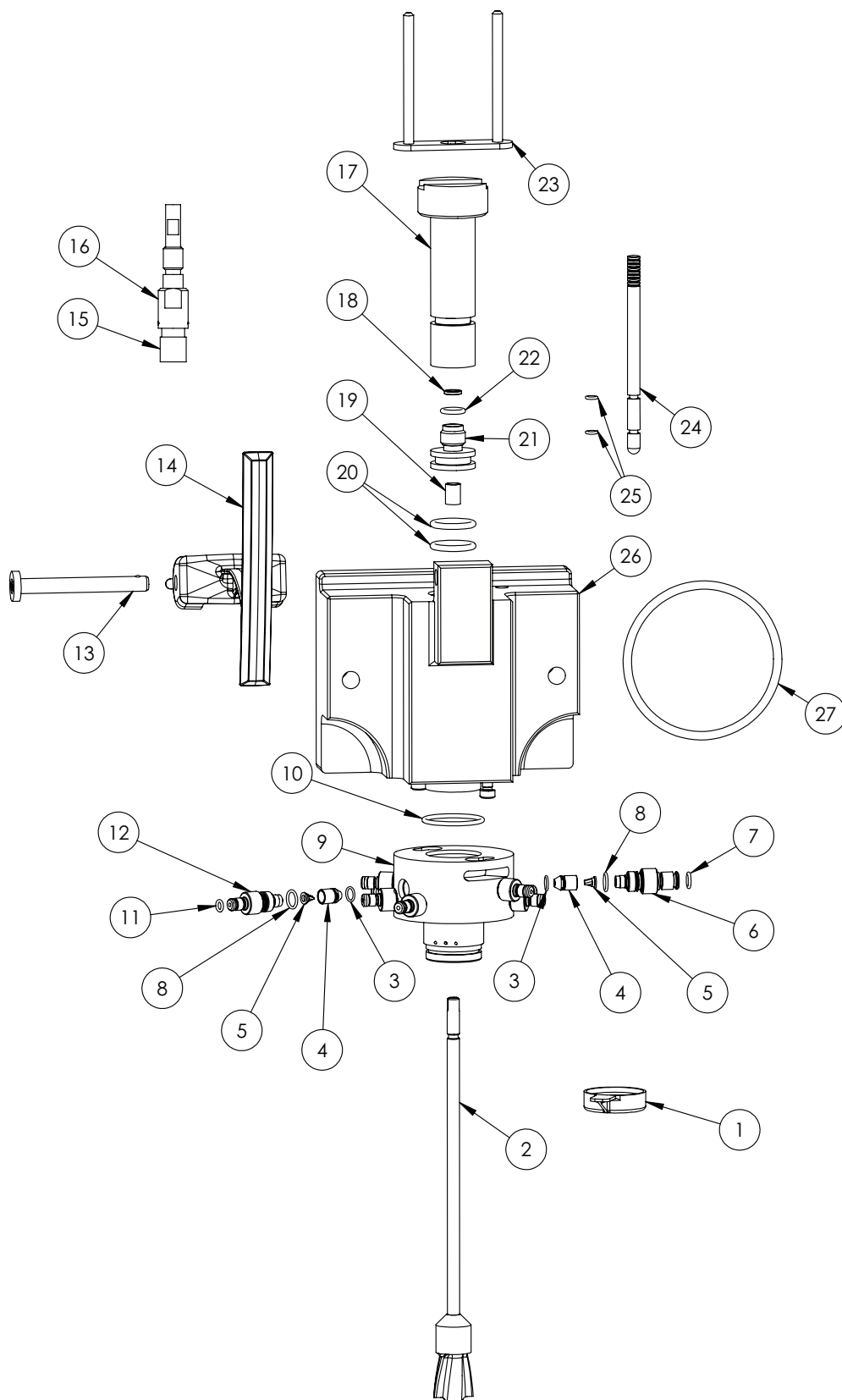
Figure 1 Head Assembly
