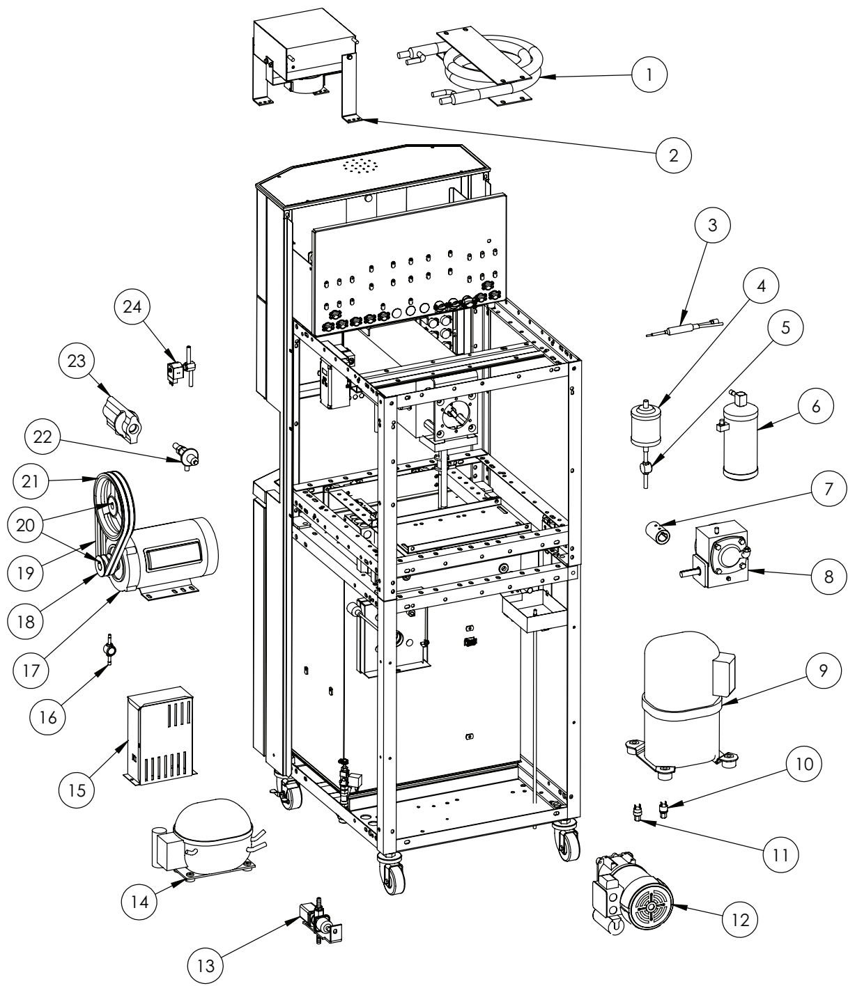
Figure 10 Water Cooled Assembly
