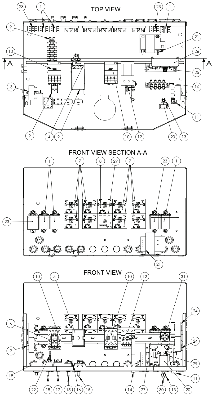
Figure 8 Electric Box
