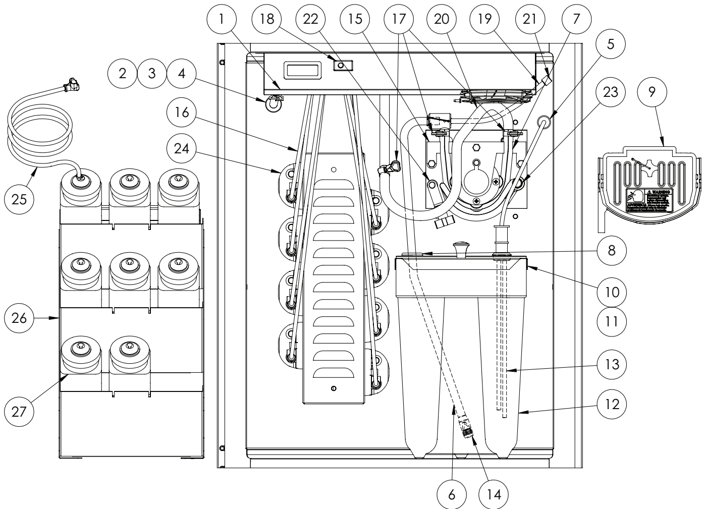
Figure 4 Cabinet Parts
