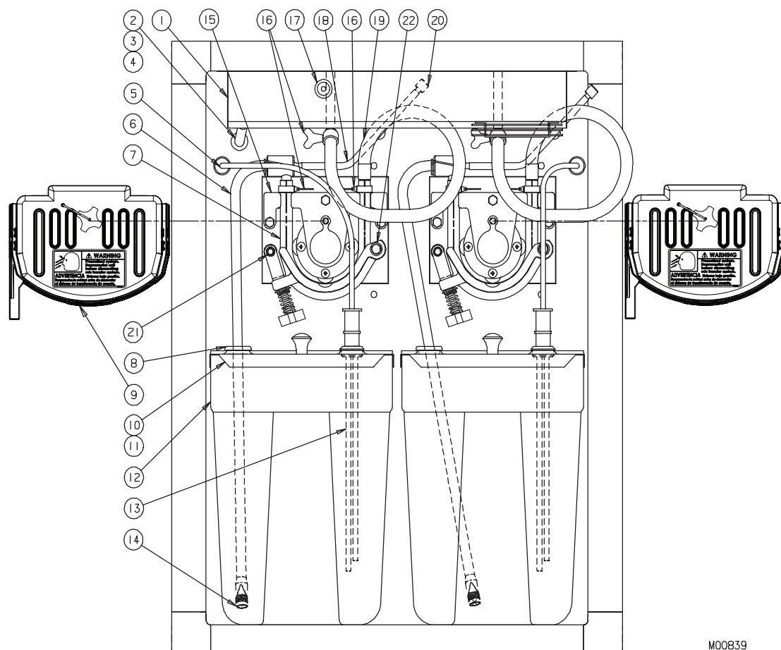
Figure 6 Cabinet Parts
