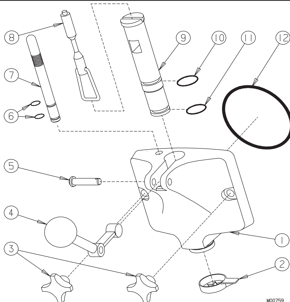
Figure 1 Head Assembly
