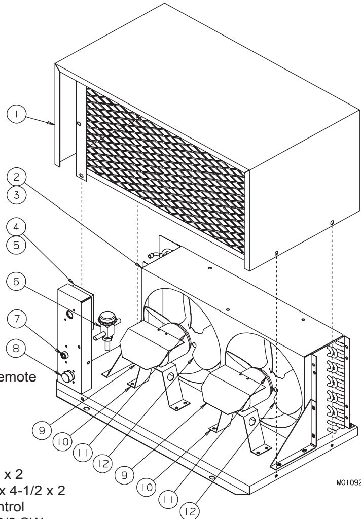
Figure 16 Air Cooled Remote Condenser
