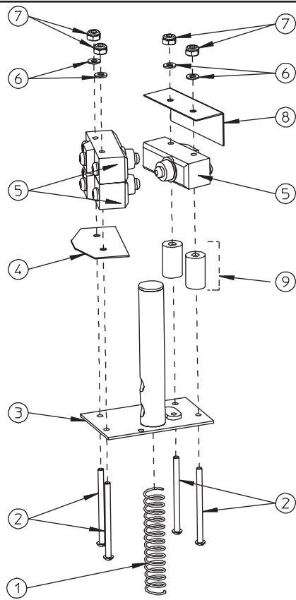
Figure 5 Switch Assembly
