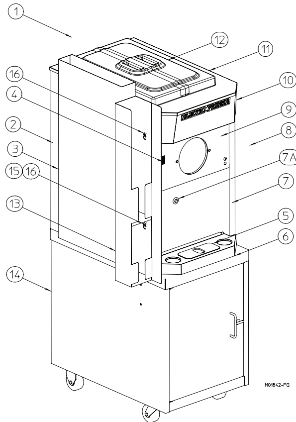
Figure 9 Panel View
