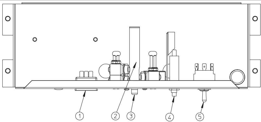
Figure 4 Plunger Box
