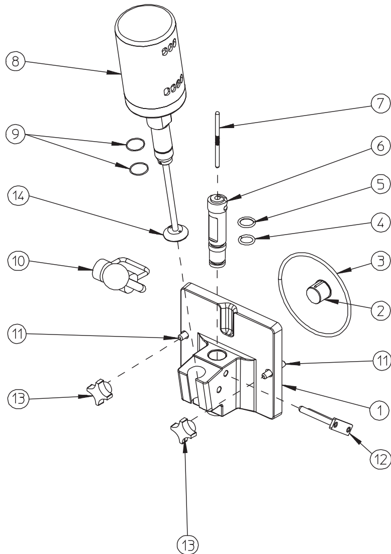
Figure 1 Head Assembly
