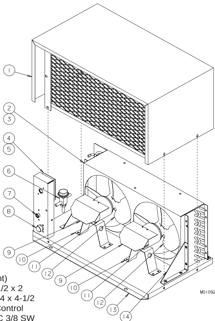
Figure 14 Air Cooled Remote Condenser
