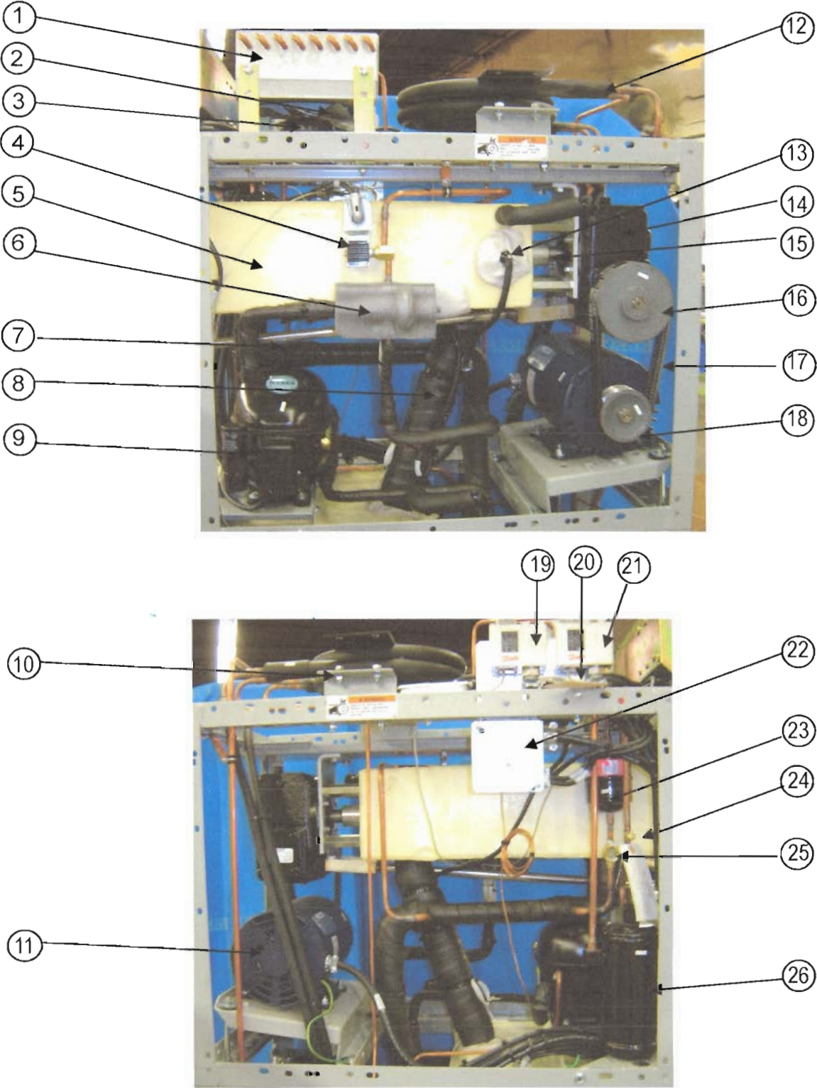
Figure 9 Water Cooled & Air Cooled Remote Assembly * (sheet 1 of 2)
