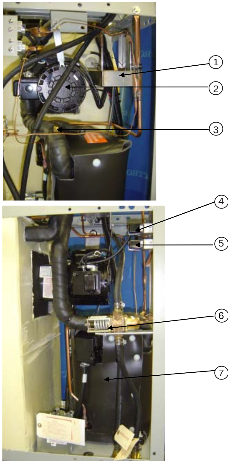
Figure 11 Cabinet Assembly* (sheet 1 of 2)
