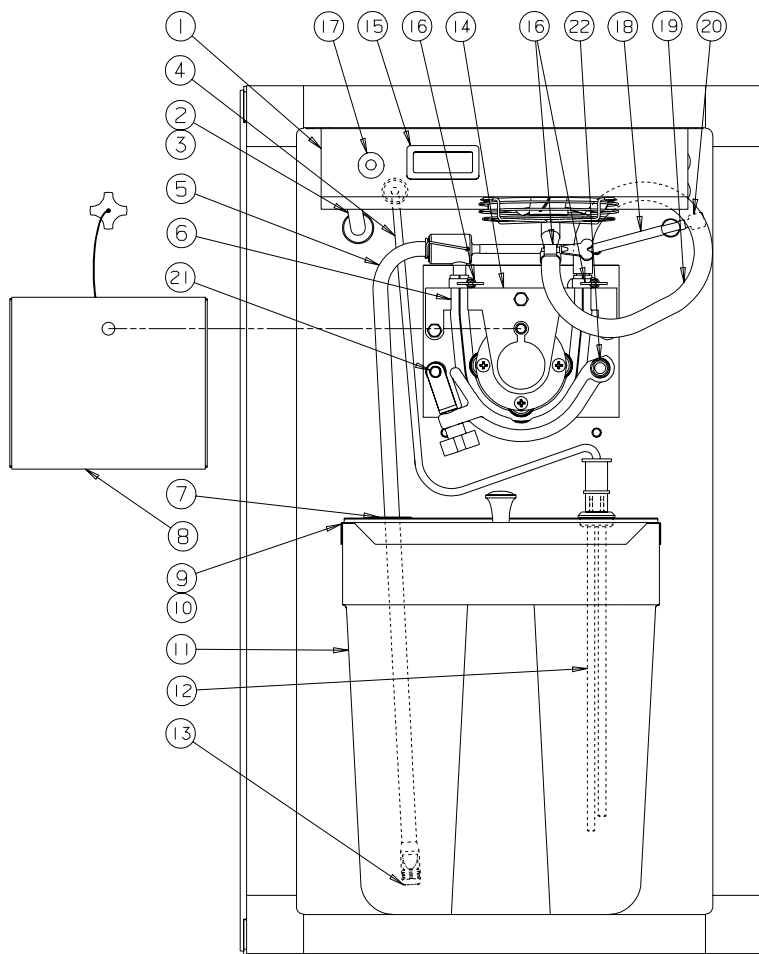
Figure 5 Cabinet Parts
