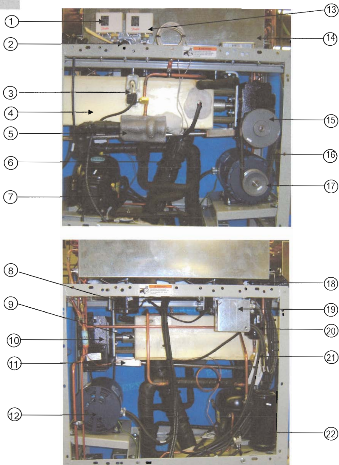
Figure 10 Air Cooled Assembly* (sheet 1 of 2)
