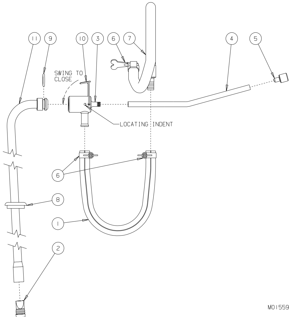
Figure 3 MTS—RMT Hose Assembly
