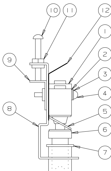
Figure 6 Spigot Switch Assembly
