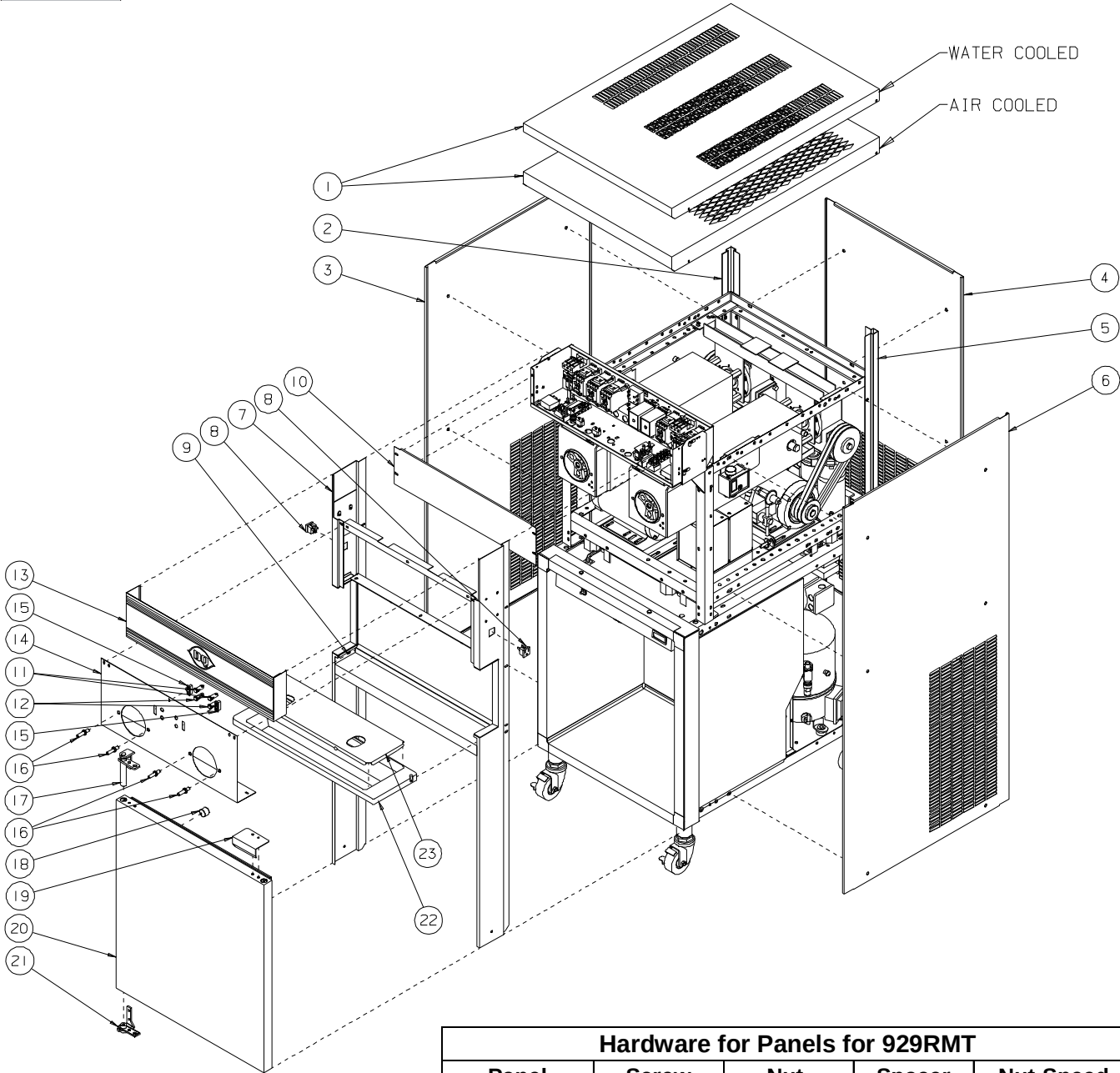
Figure 9 929RMT Panel Assembly (sheet 1 of 2)
