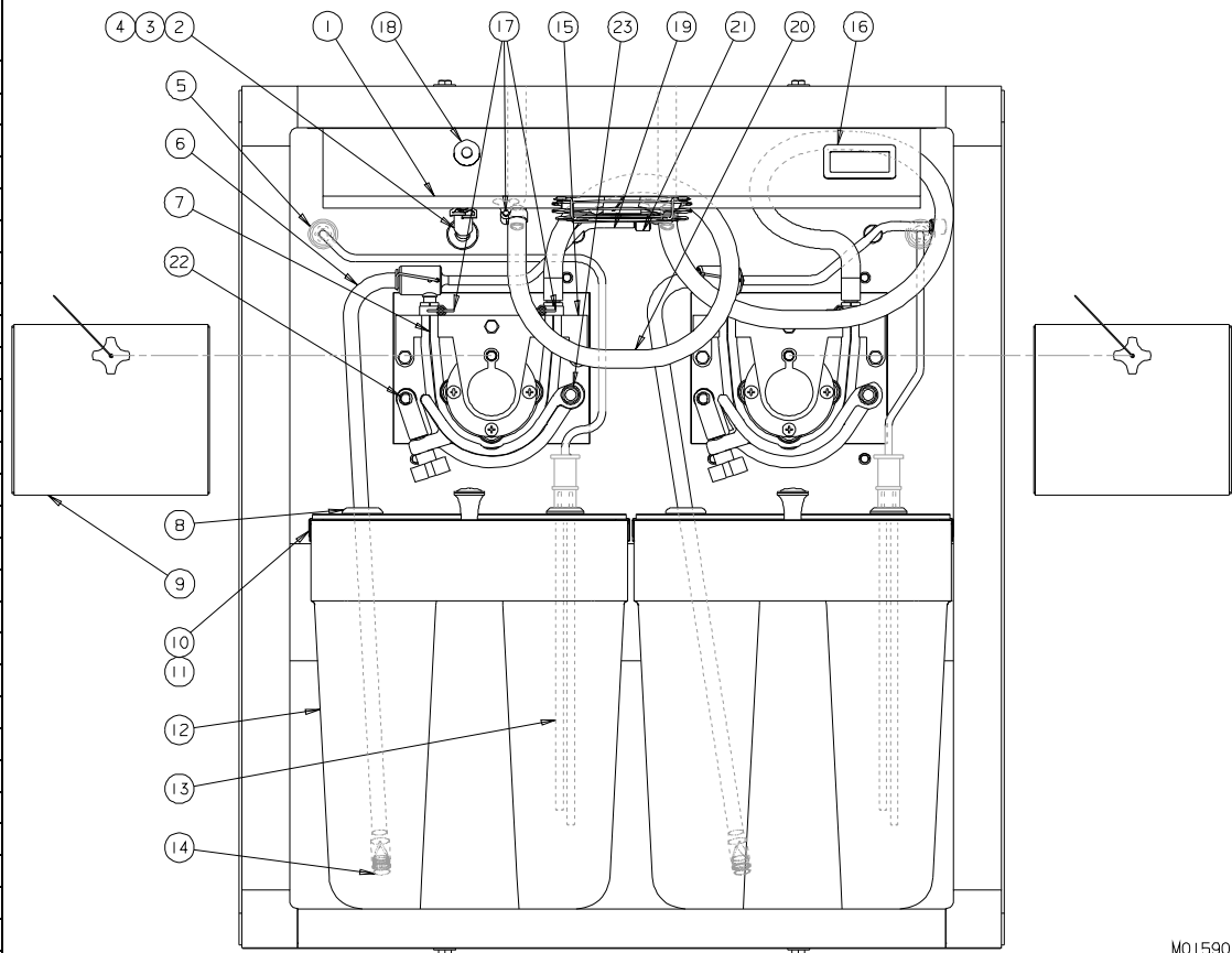
Figure 5 Cabinet Parts
