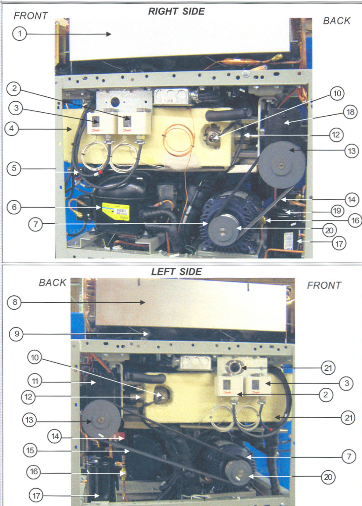
Figure 9 Upper Side Views (sheet 2 of 2)
