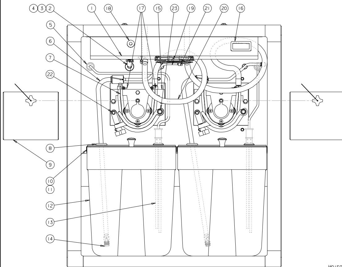
Figure 5 Cabinet Parts
