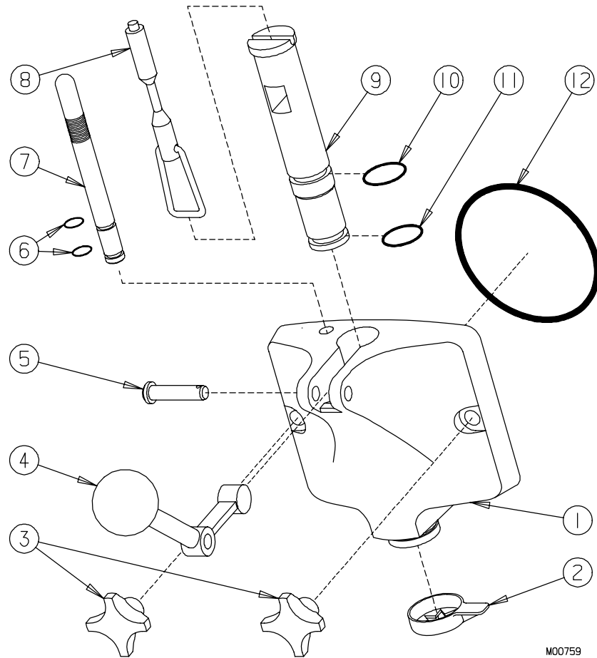
Figure 1 Head Assembly
