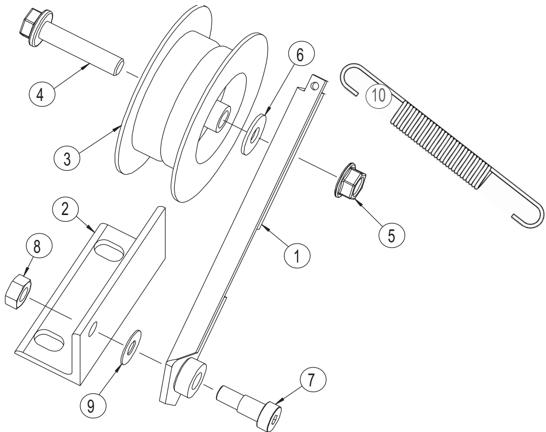
Figure 7 Idler Pulley Assembly
