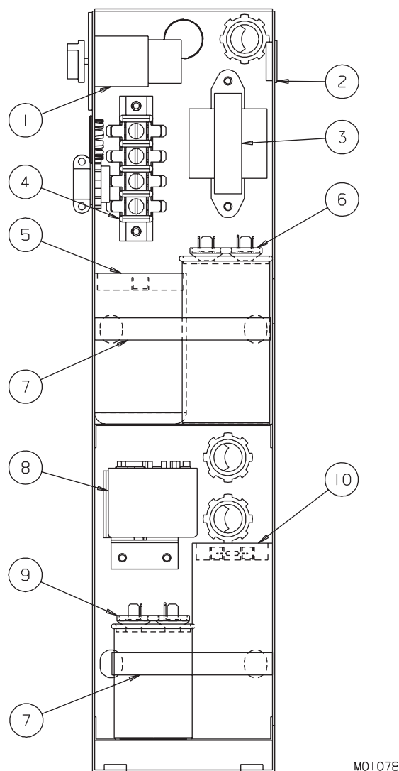
Figure 5 Capacitor/Relay Box
