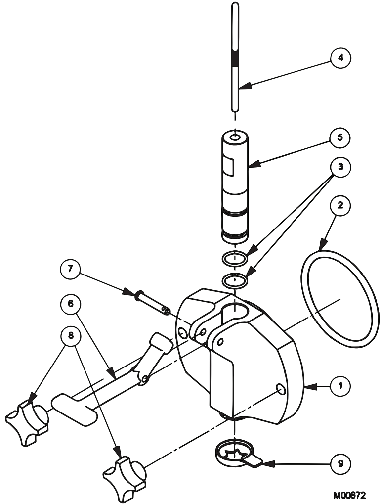
Figure 1 Head Assembly
