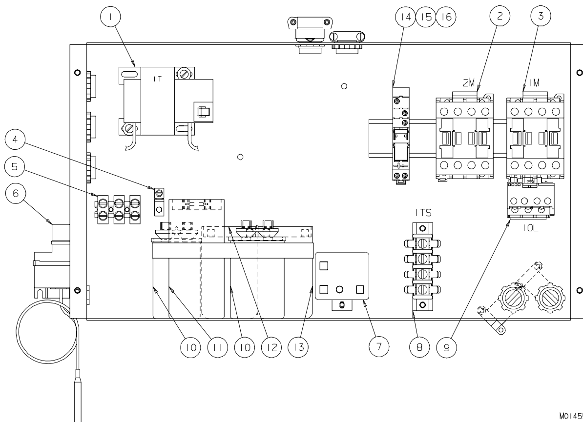
Figure 10 Electric Box
