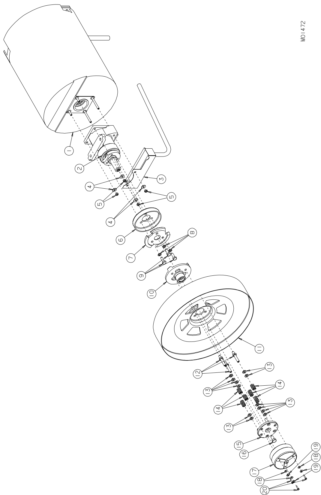
Figure 8 Drive Assembly (Sheet 1 of 2)
