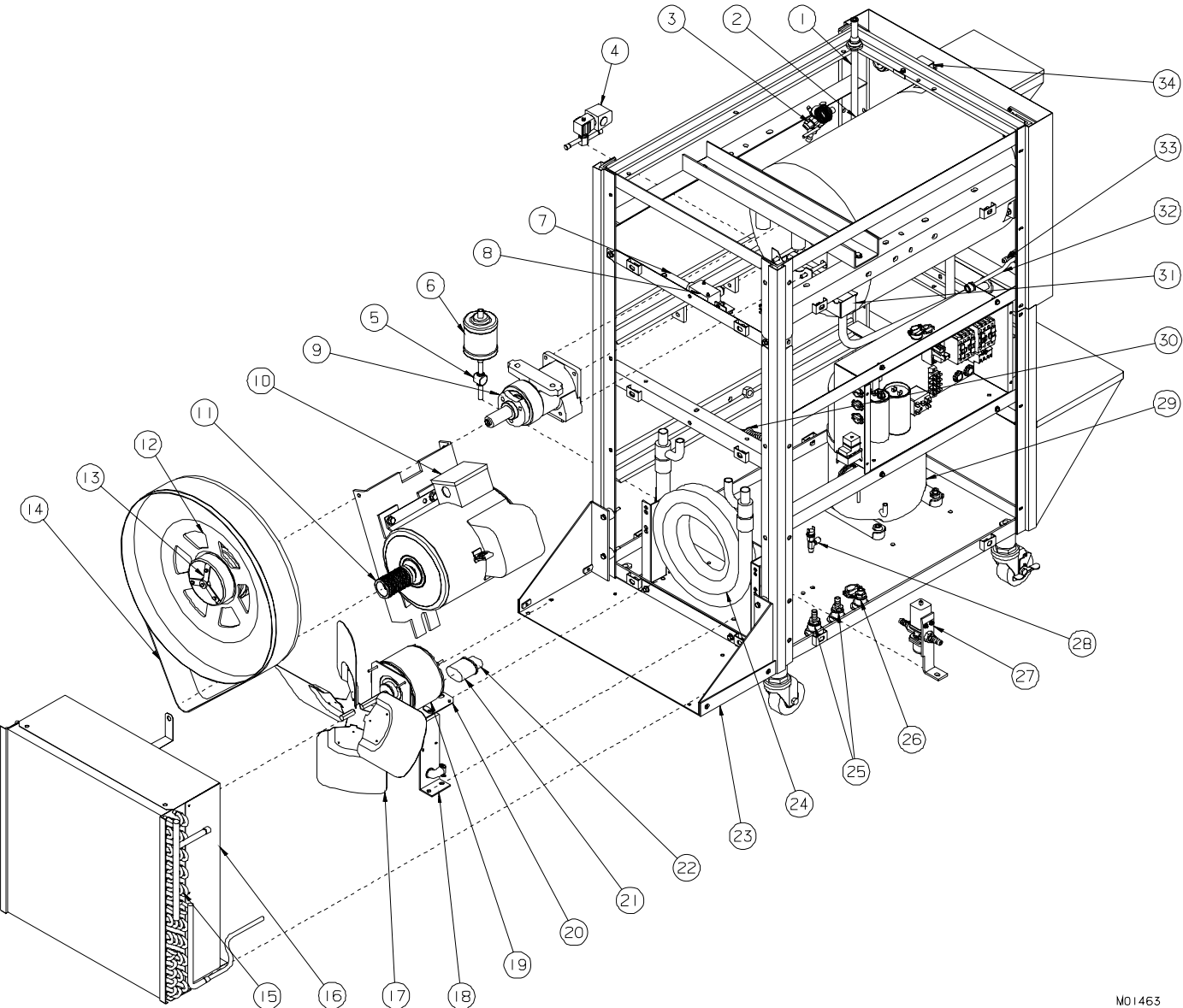
Figure 7 B24 Rear View (Sheet 1 of 2)
