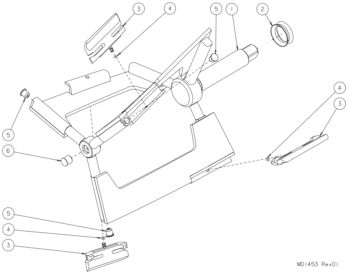
Figure 2 B12 Dasher Assembly
