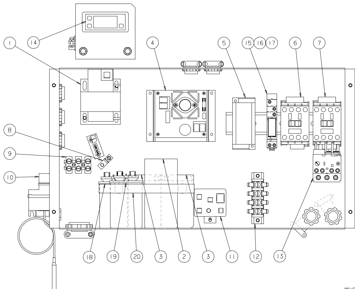
Figure 4 Electric Box RFC3
