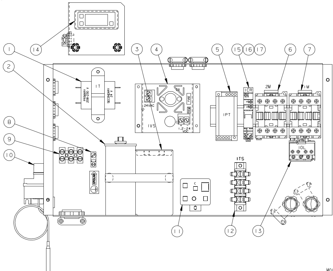
Figure 5 Electric Box RFC5
