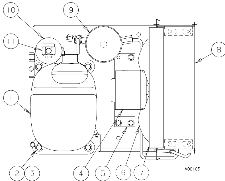
Figure 9 Condensing Unit Assembly-Air Cooled
