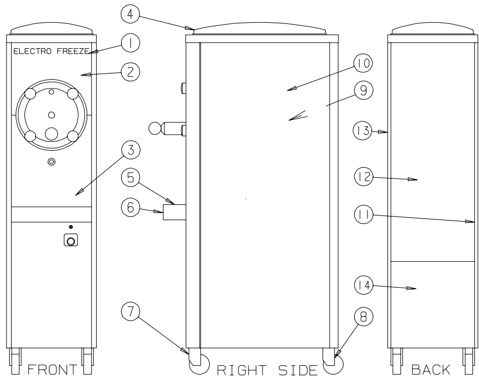
Figure 12 Panels — Floor Models
