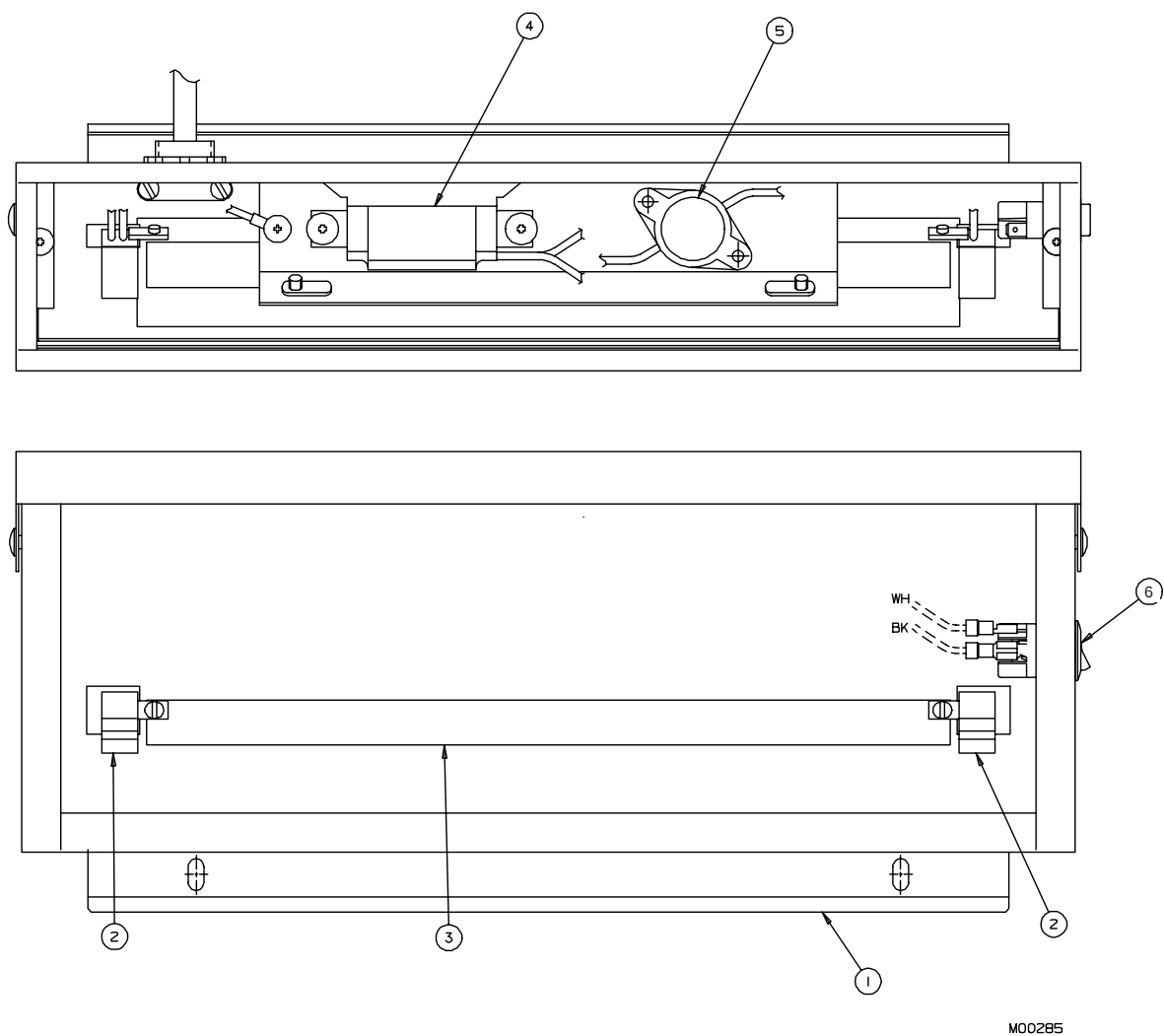
Figure 13 Accessory - Merchandiser (Optional - Floor Models Only)
