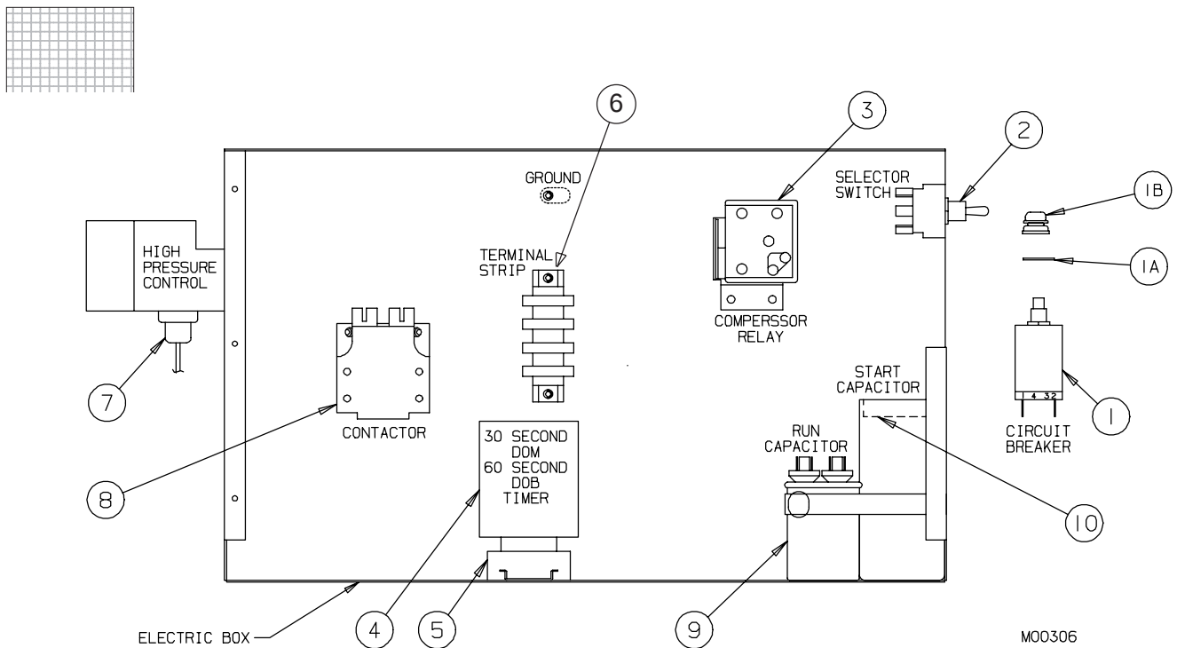
Figure 5 Electrical Box — Counter Model
