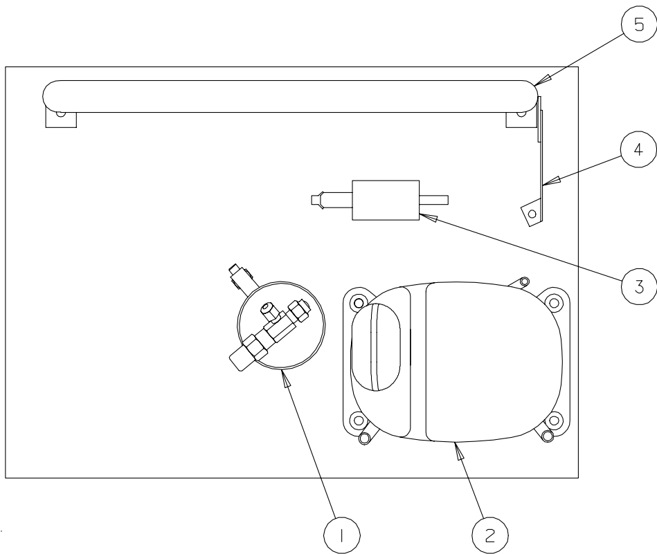
Figure 10 Condensing Unit Assembly - Water Cooled
