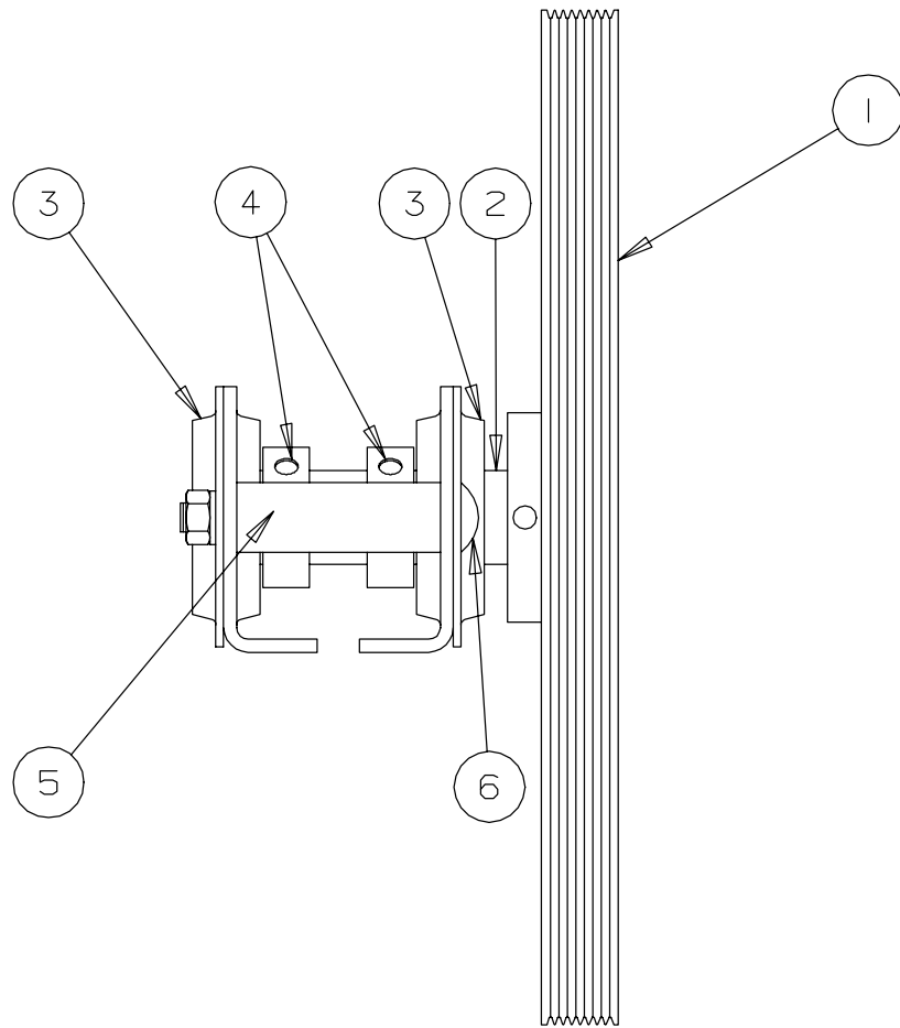
Figure 7 Drive Shaft and Bearing Assembly
