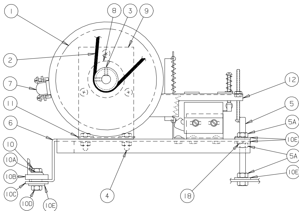
Figure 8 Motor and Bearing Assembly
