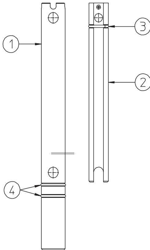
Figure 3 Mix Feed Tube Assembly
