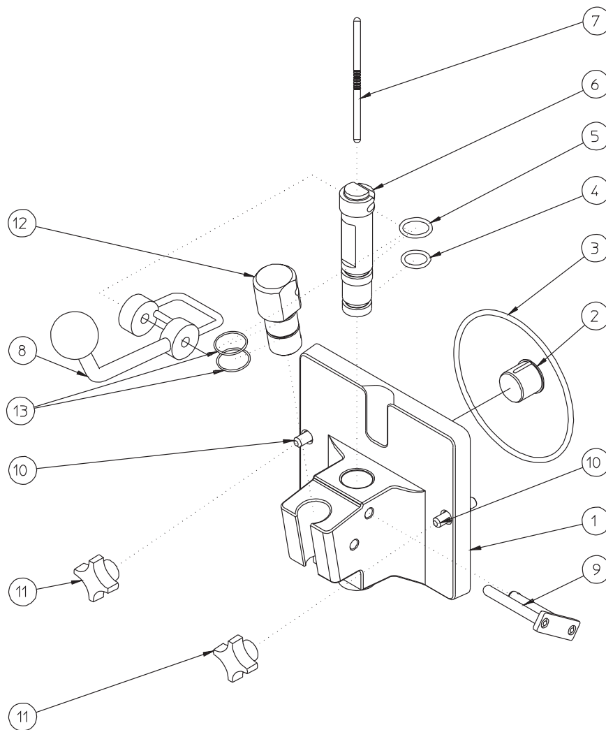
Figure 1 Head Assembly
