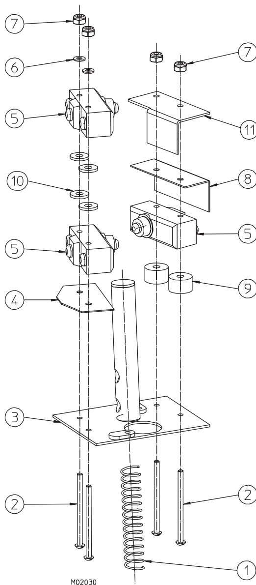
Figure 5 Switch Assembly
