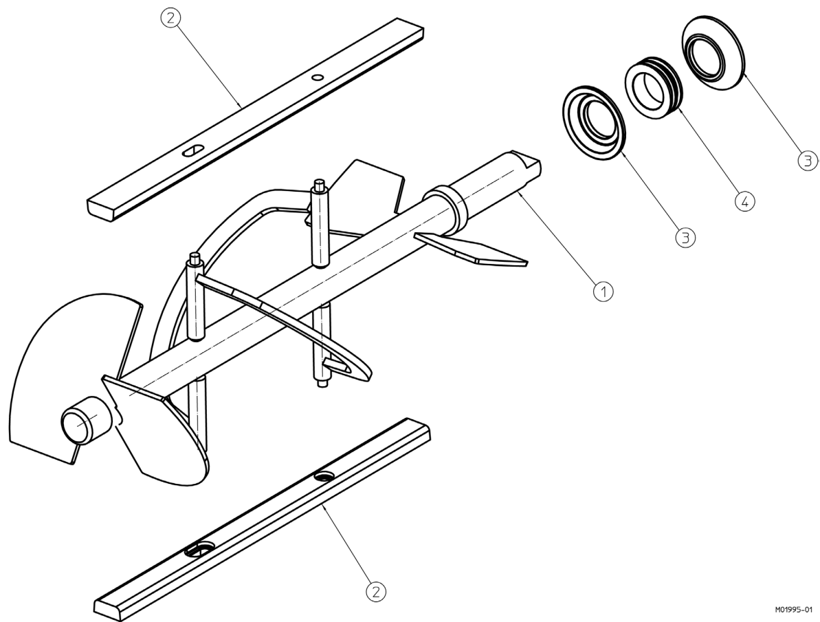
Figure 2 Beater Shaft Assembly
