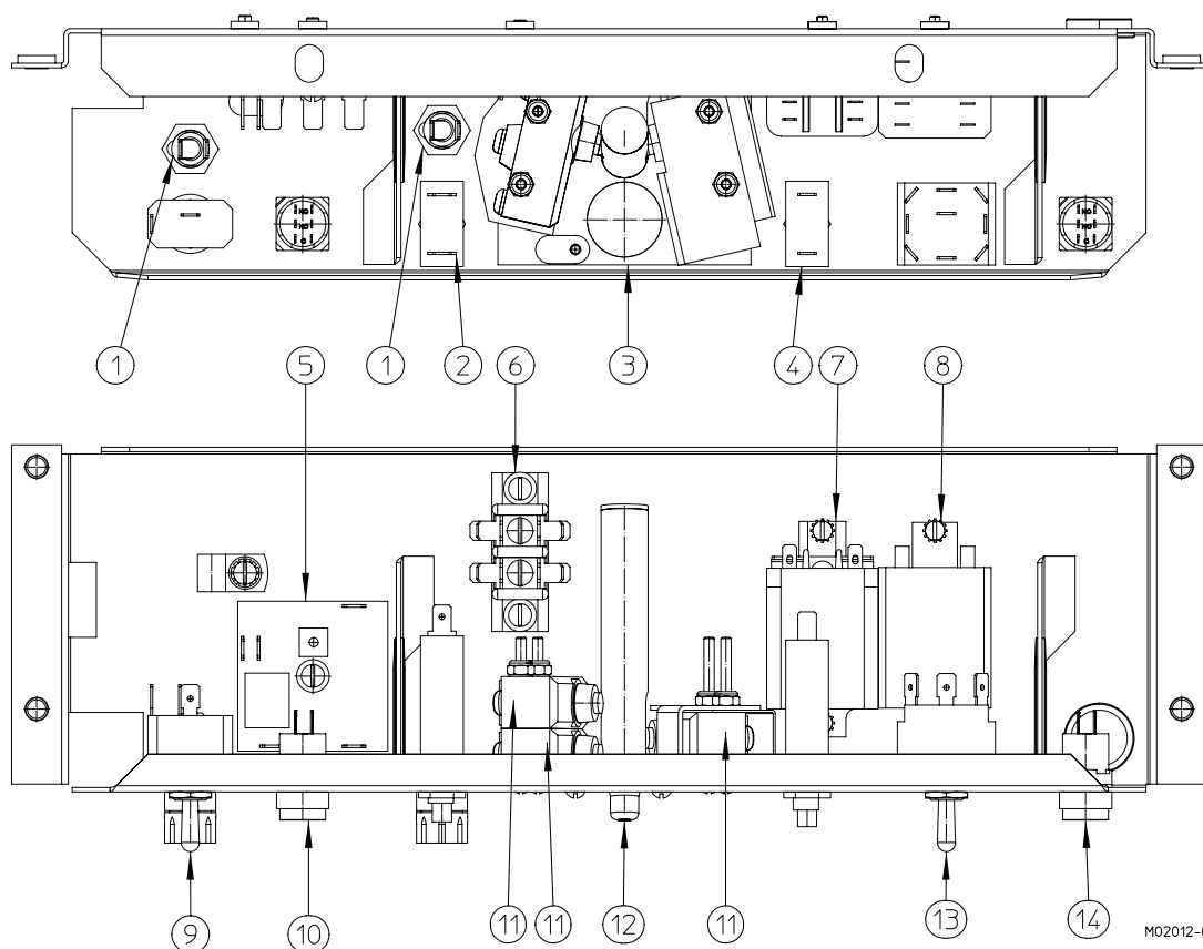
Figure 4 Plunger Box
