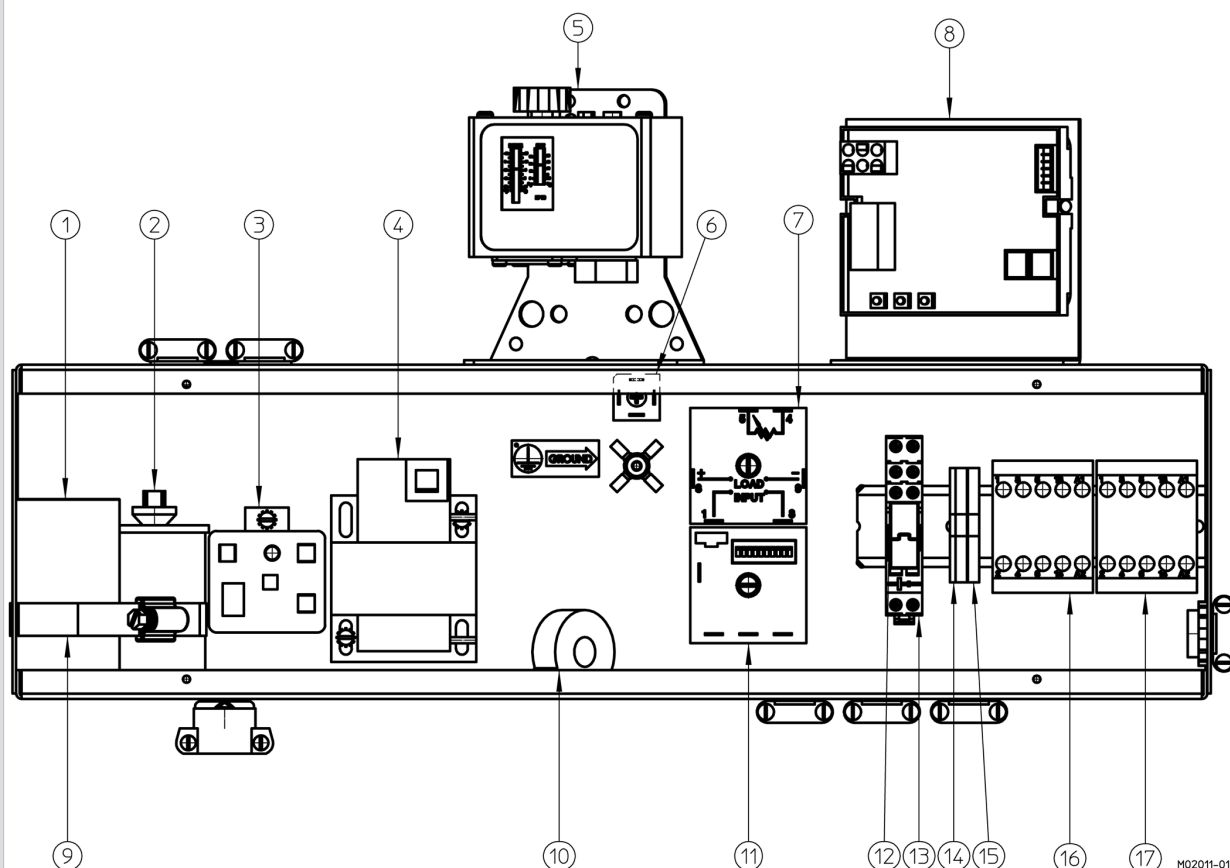
Figure 6 Electrical Box
