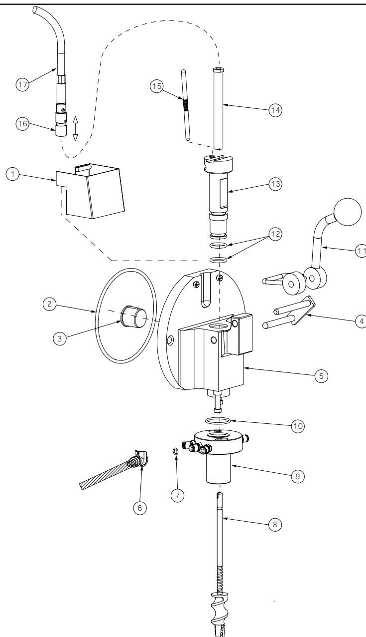
Figure 1 Head Assembly
