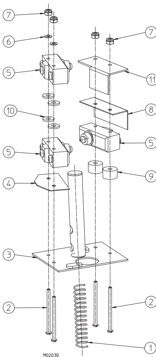
Figure 4 Switch Assembly
