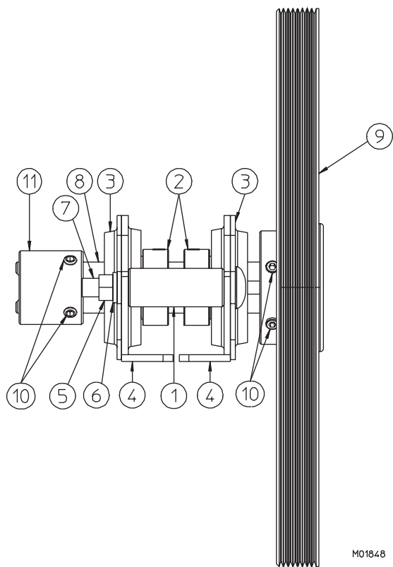
Figure 9 Drive Shaft and Bearing Assembly
