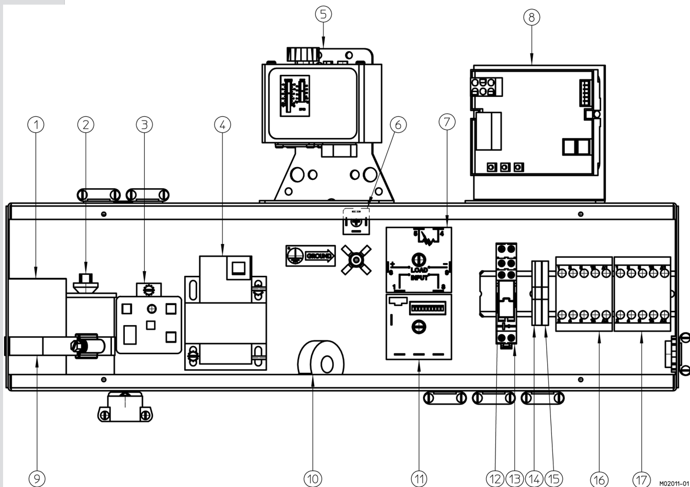
Figure 6 Electrical Box
