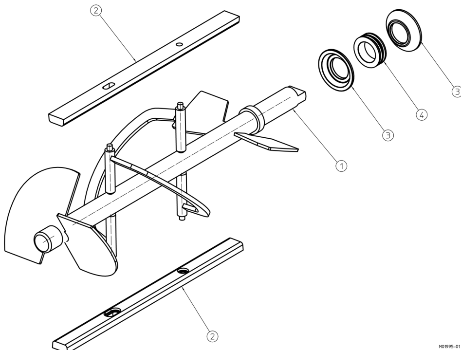
Figure 2 Beater Shaft Assembly
