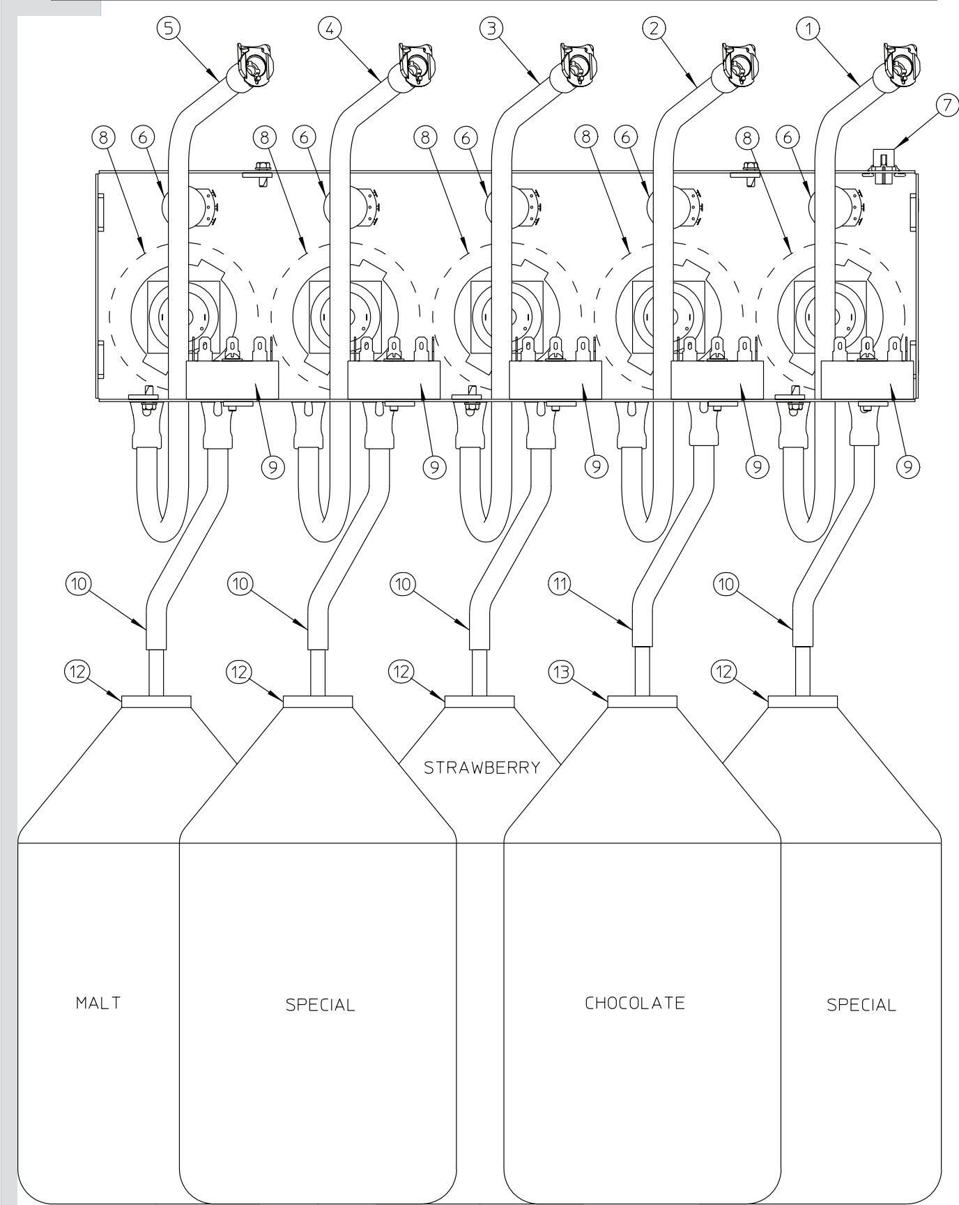
Figure 7 Syrup System View (Sheet 1 of 2)
