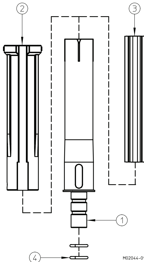
Figure 4 Mix Feed Tube Assembly
