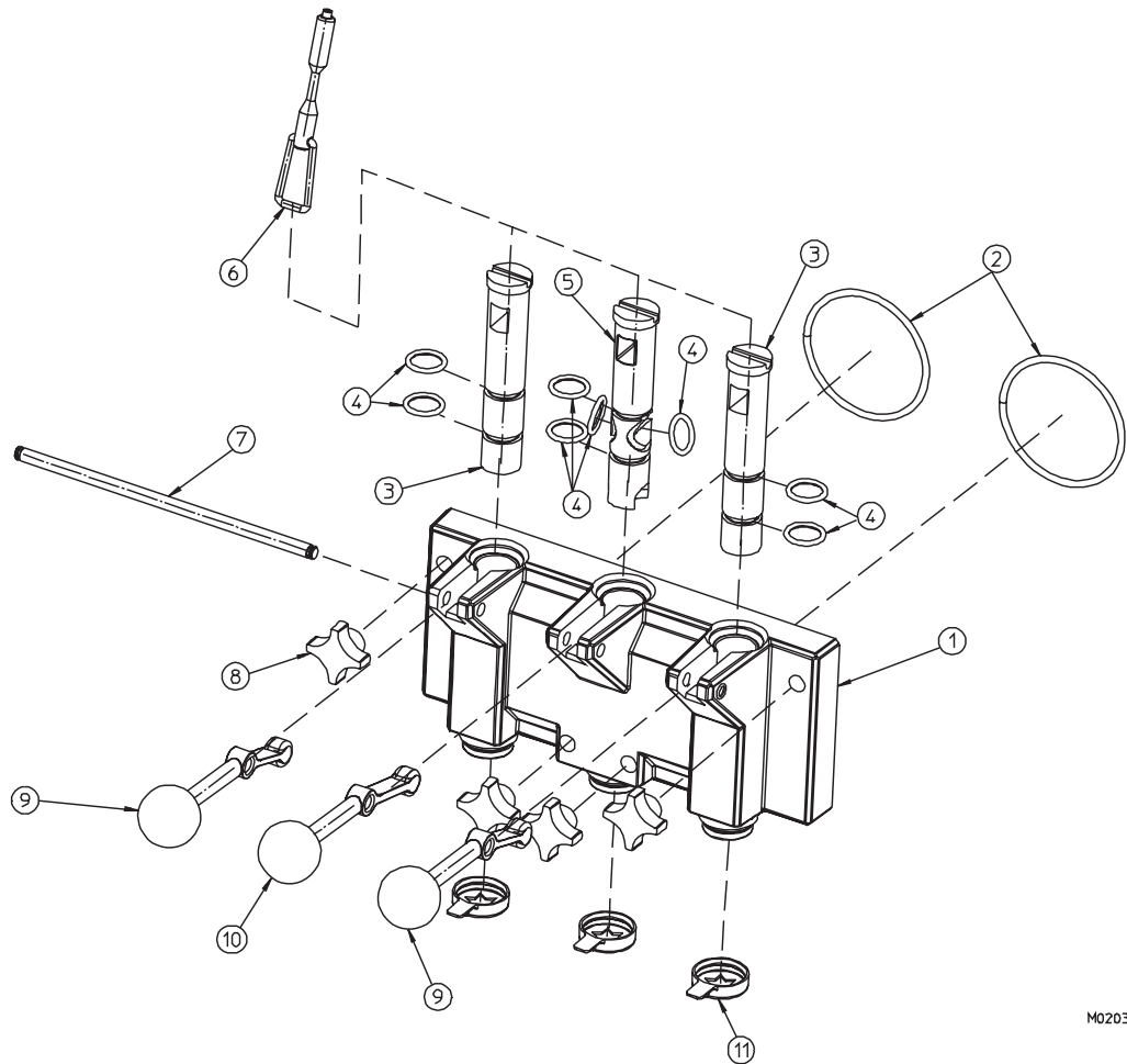
Figure 1 Head Assembly
