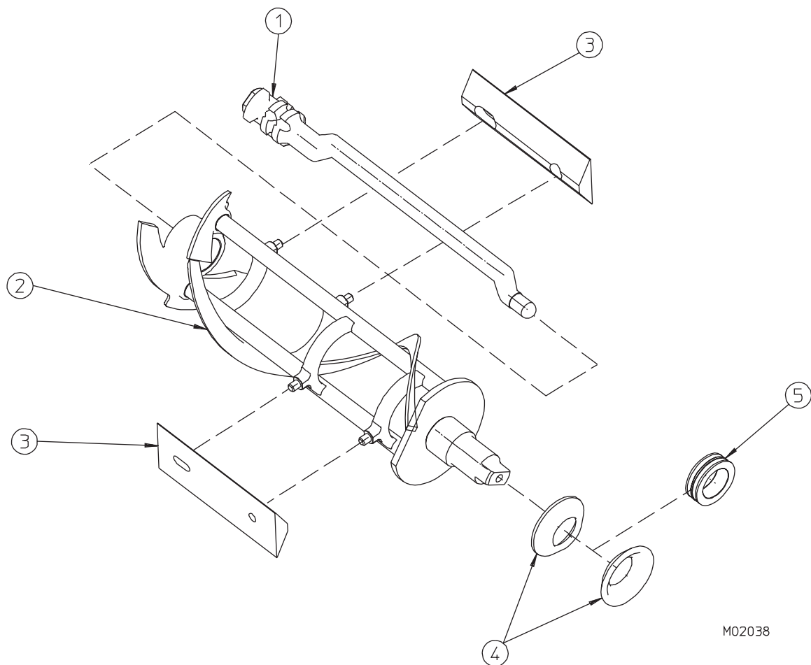
Figure 2 SLX400E Beater Shaft Assembly
