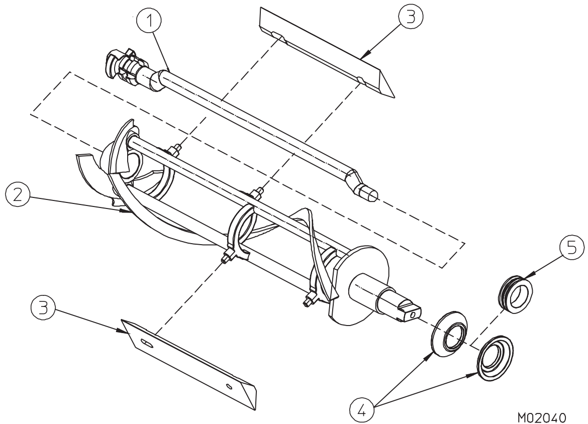
Figure 3 SLX500 Beater Shaft Assembly
