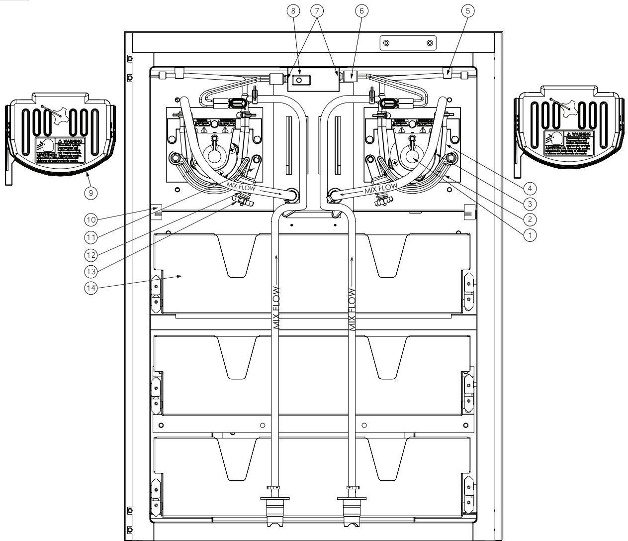
Figure 3 Cabinet Parts
