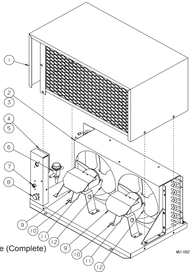
Figure 16 Air Cooled Remote Condenser
