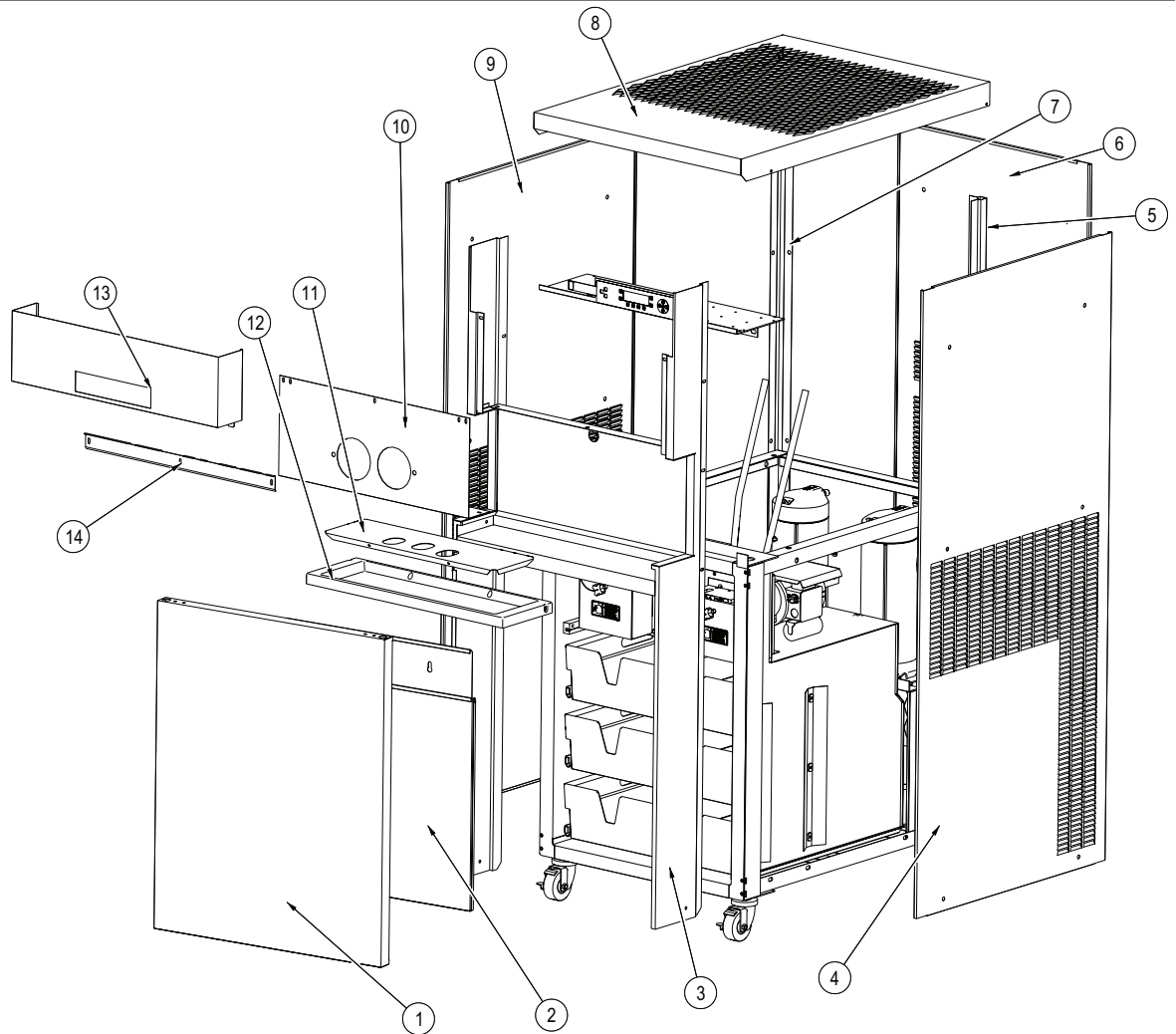
Figure 12 Panel Breakdown
