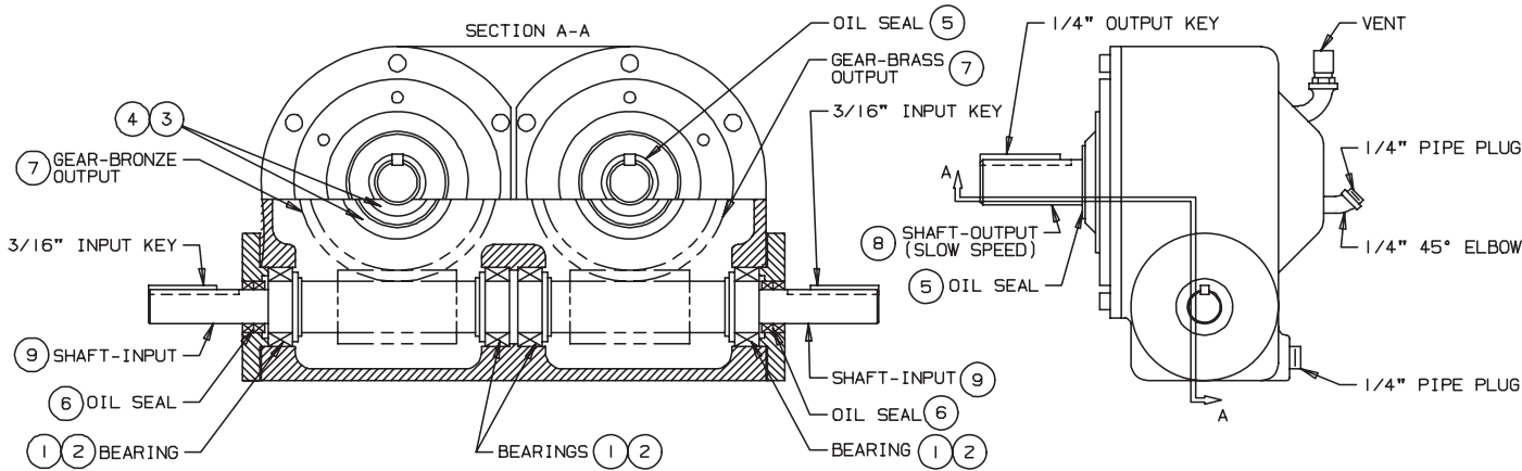
Figure 14 Gear Reducer
