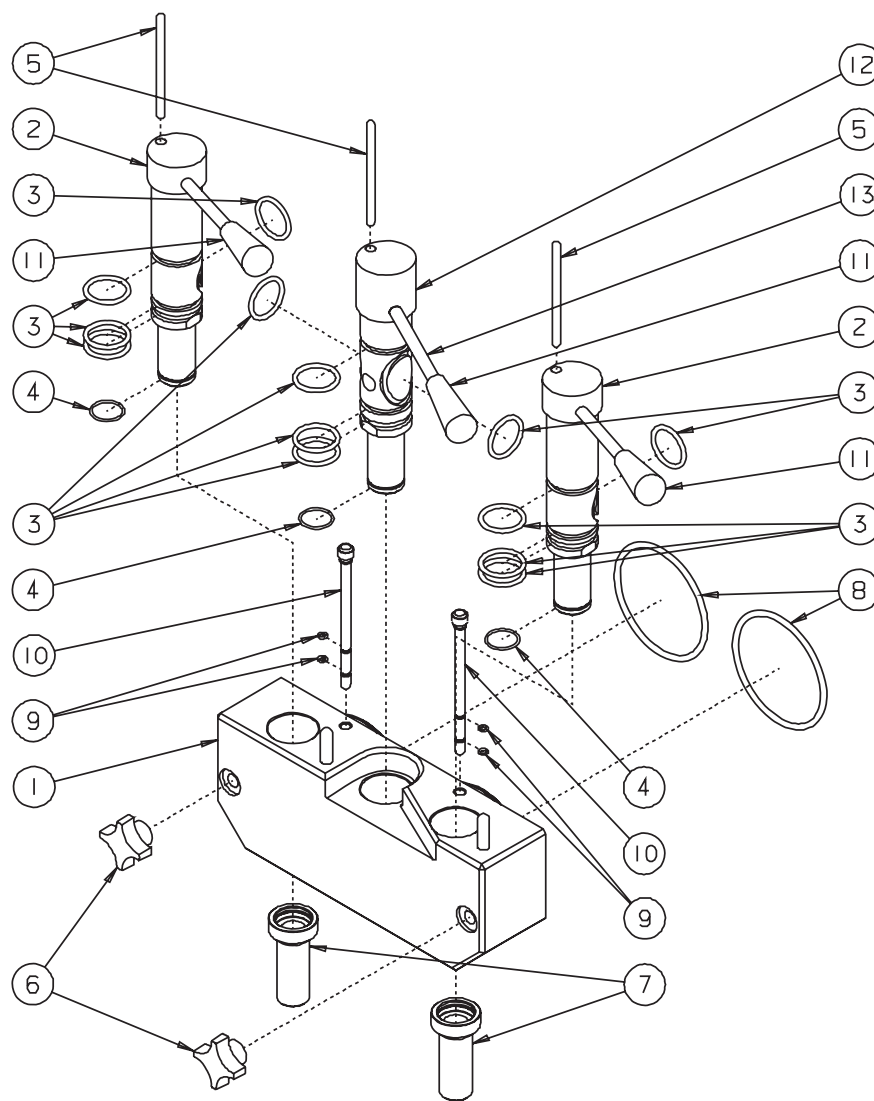
Figure 1 Head Assembly
