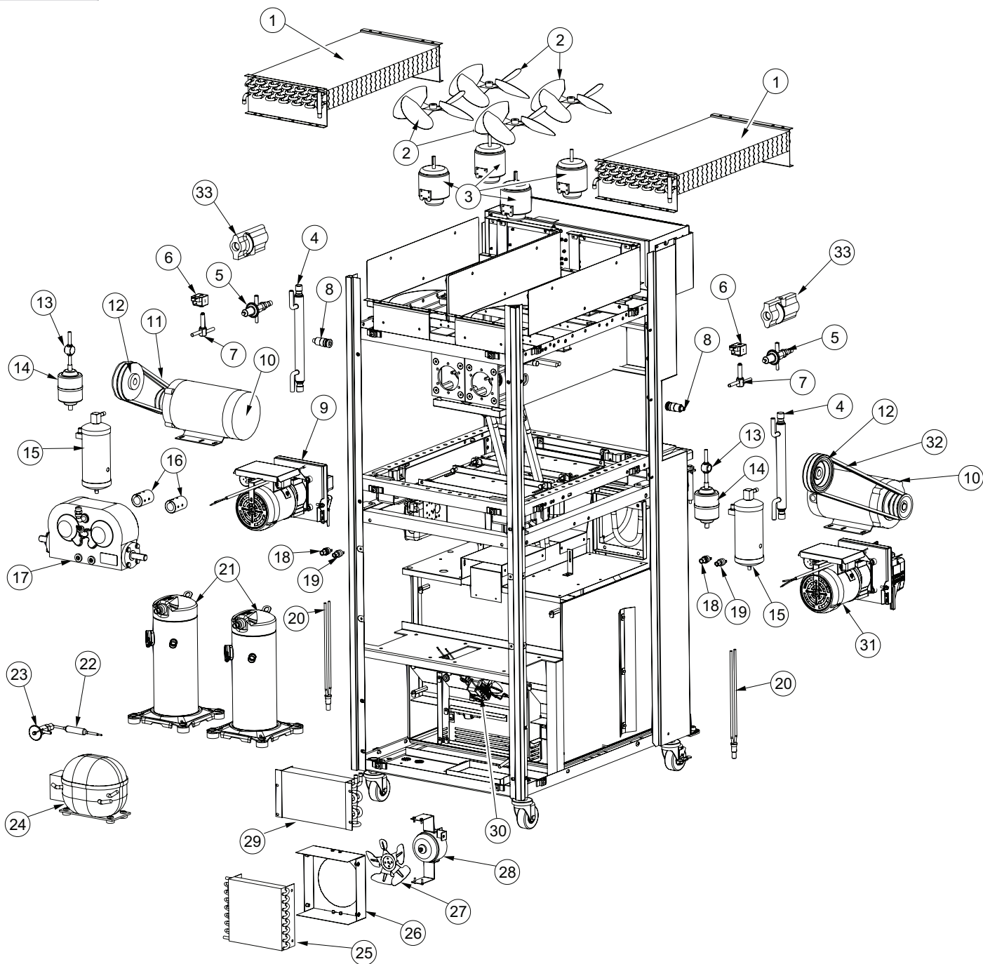
Figure 11 Air Cooled Side/Back View (Breakdown)
