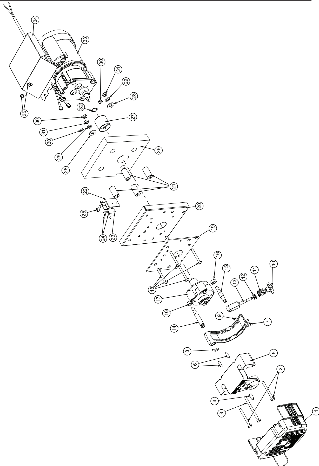
Figure 5 Mix Transfer System RMT 1Ph. (Sheet 1 of 2)
