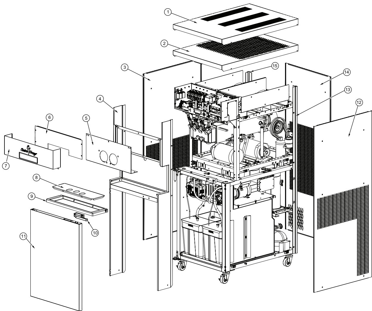
Figure 10 Panel Breakdown (Breakdown)
