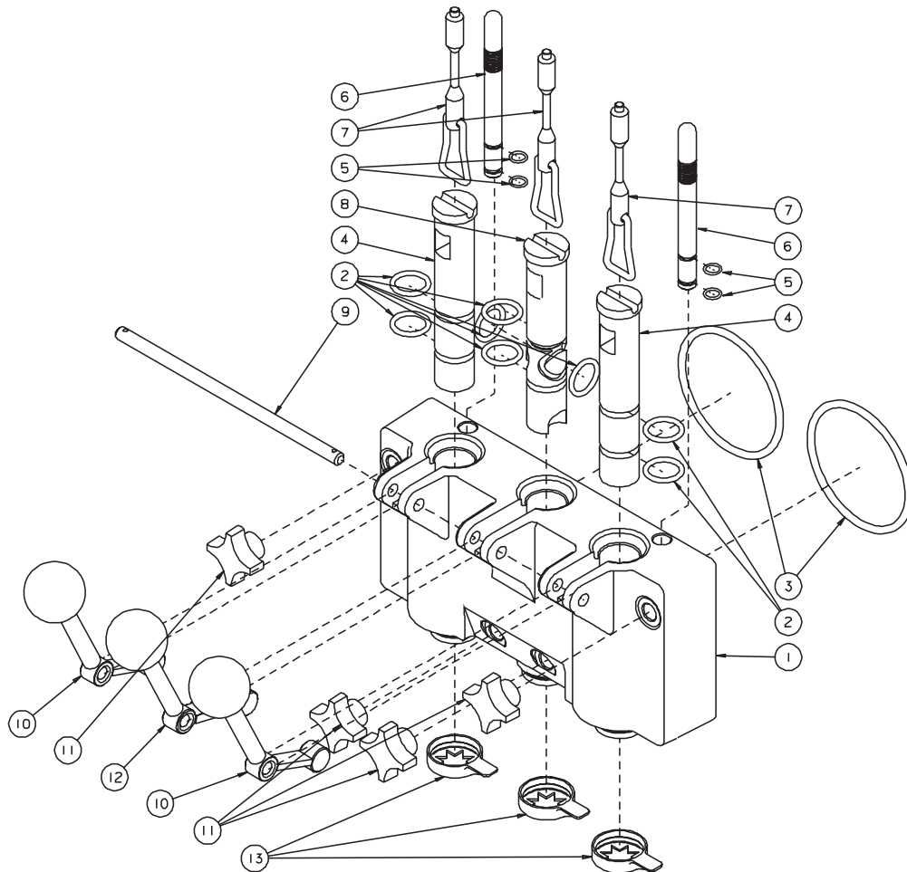
Figure 1 Head Assembly
