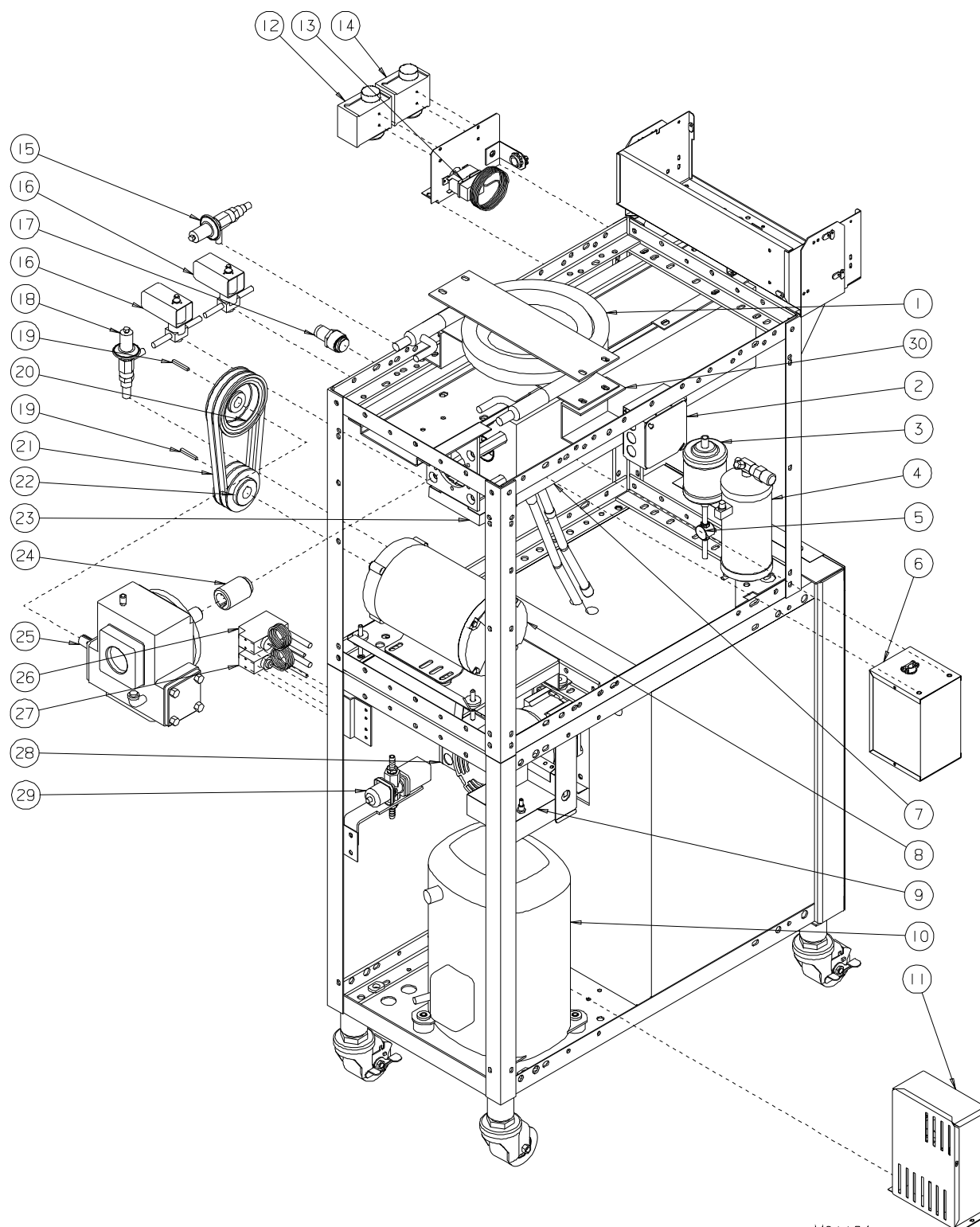
Figure 13 15N-CMT-W Water Cooled Side/Back View (Sheet 1 of 2)
