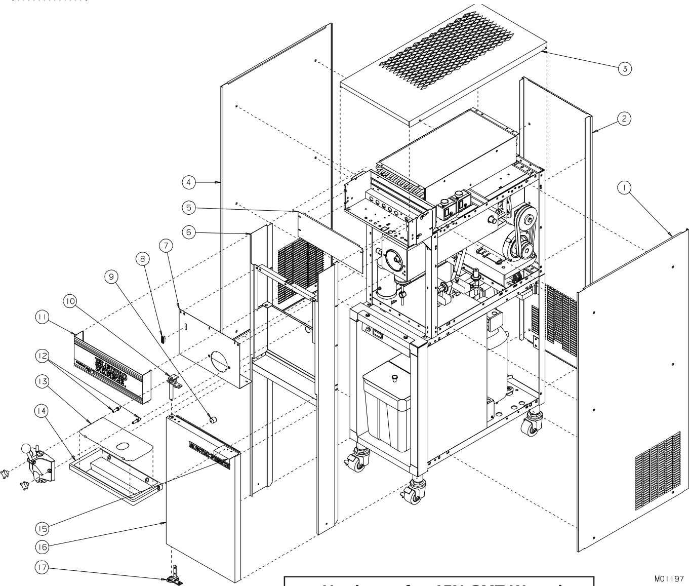
Figure 6 Panels — Air Cooled 15N-CMT-W and 44N-CMT-W (sheet 1 of 2)
