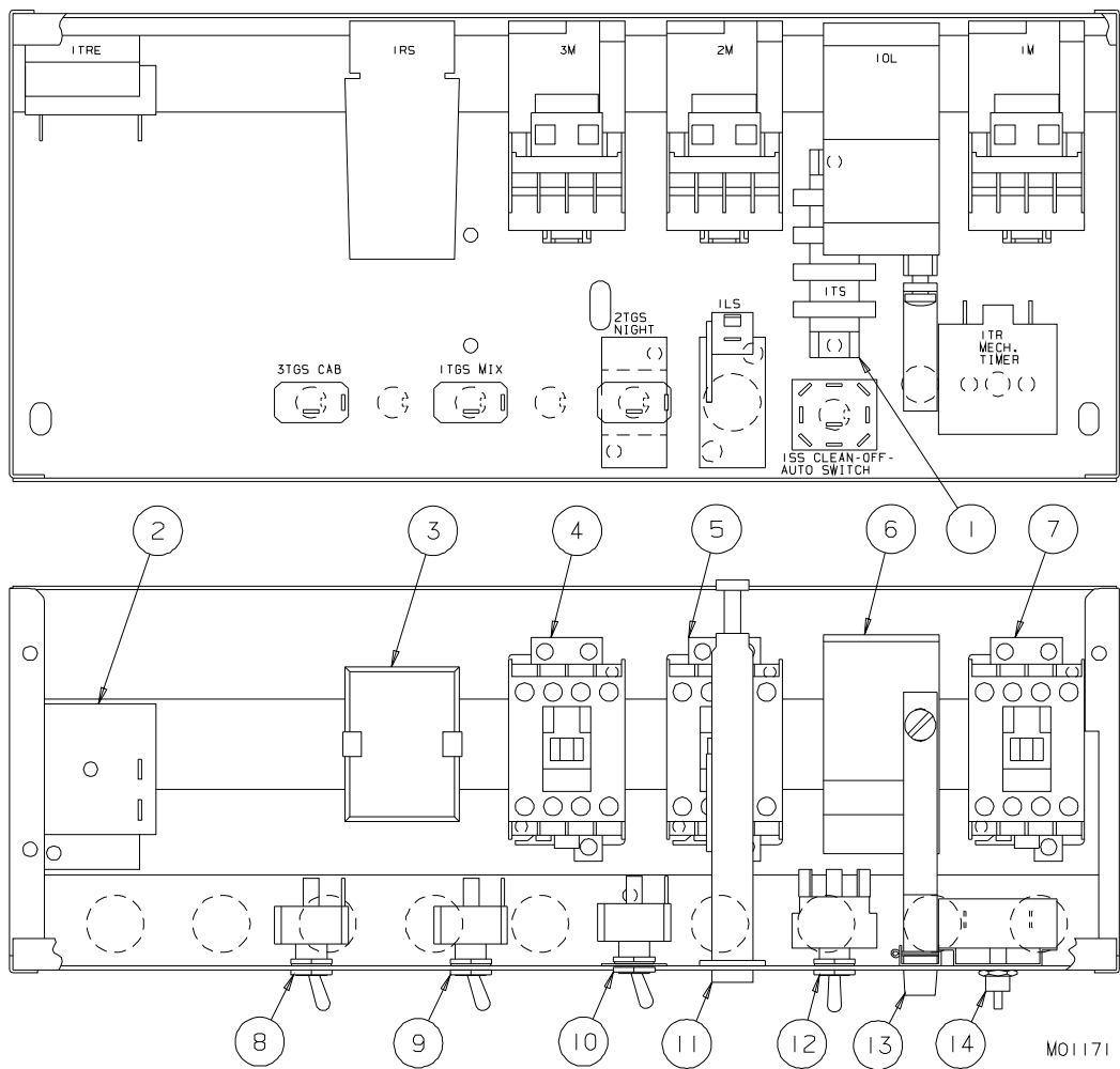
Figure 8 Switch Box — 15N-CMT-W and 44N-CMT-W
