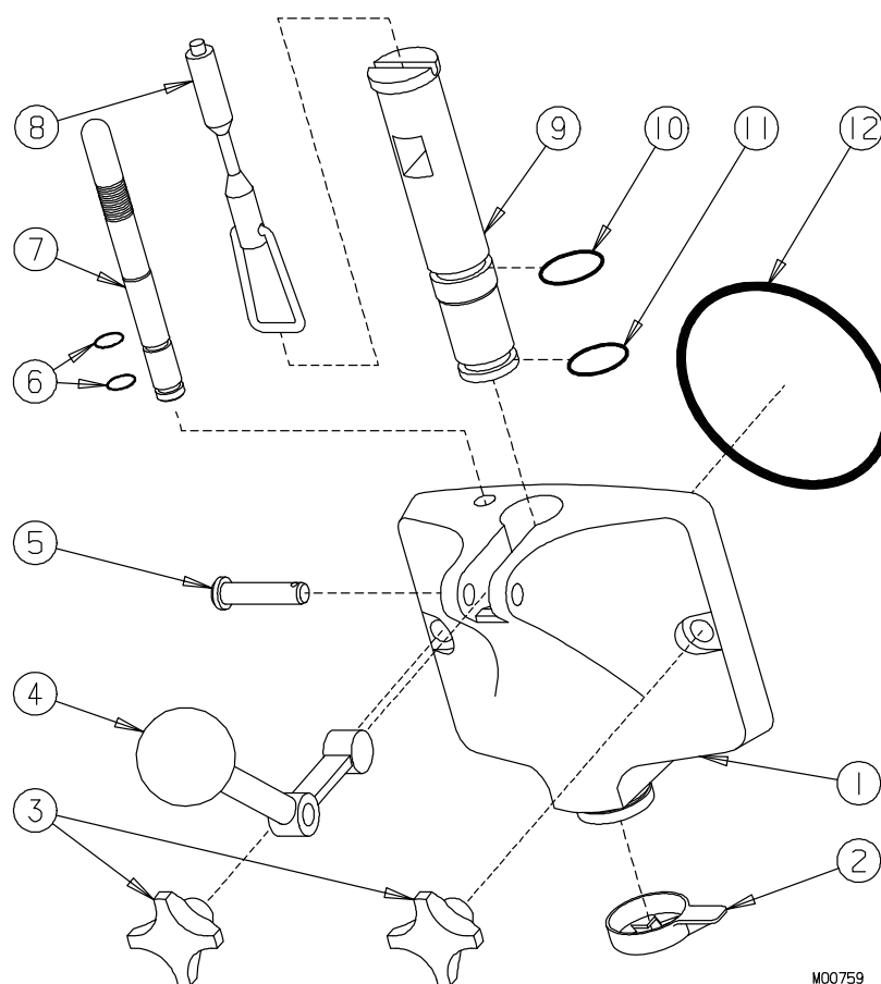
Figure 1 Head Assembly
