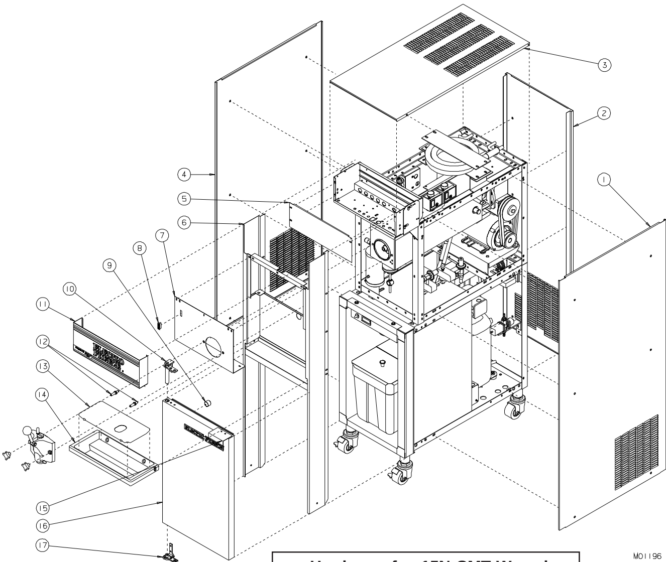
Figure 7 Panels — Water Cooled and Air Cooled Remote 15N-CMT-W and 44N-CMT-W (sheet 1 of 2)
