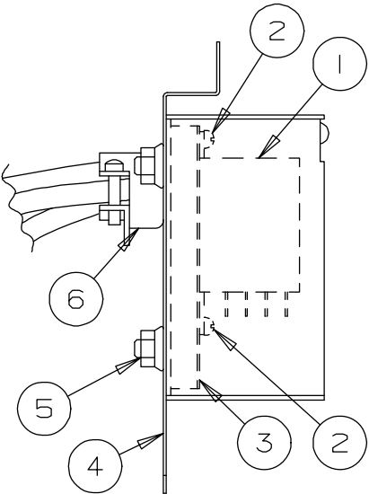
Figure 10 Relay Box — MTS 44N-CMT 3 Phase, 15N-CMT-W 1 & 3 Phase
