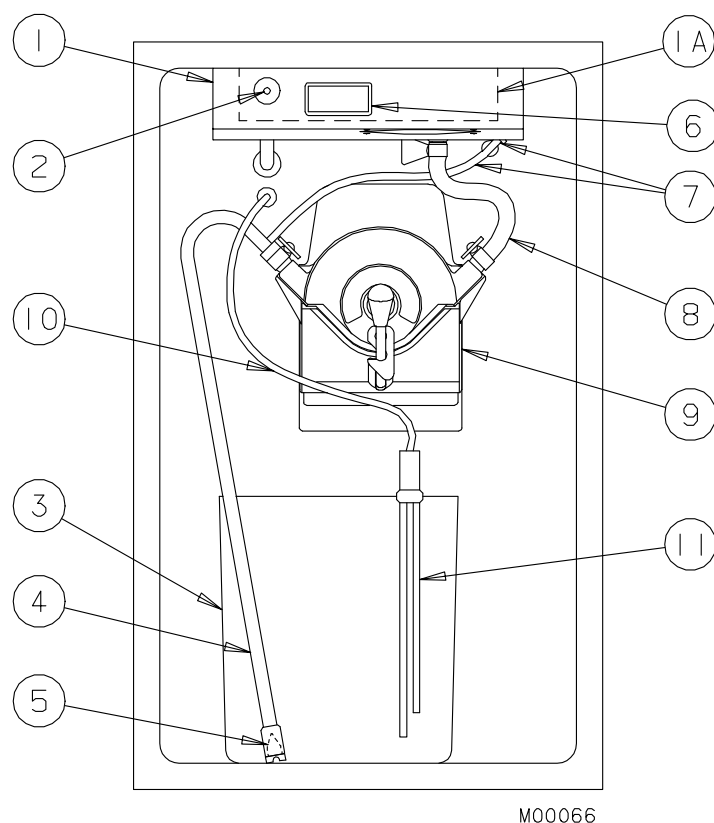
Figure 3 Cabinet Parts
