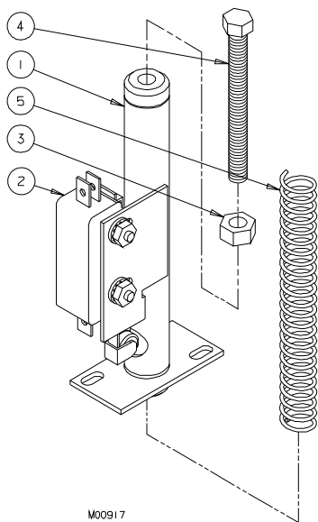
Figure 9 Switch Assembly
