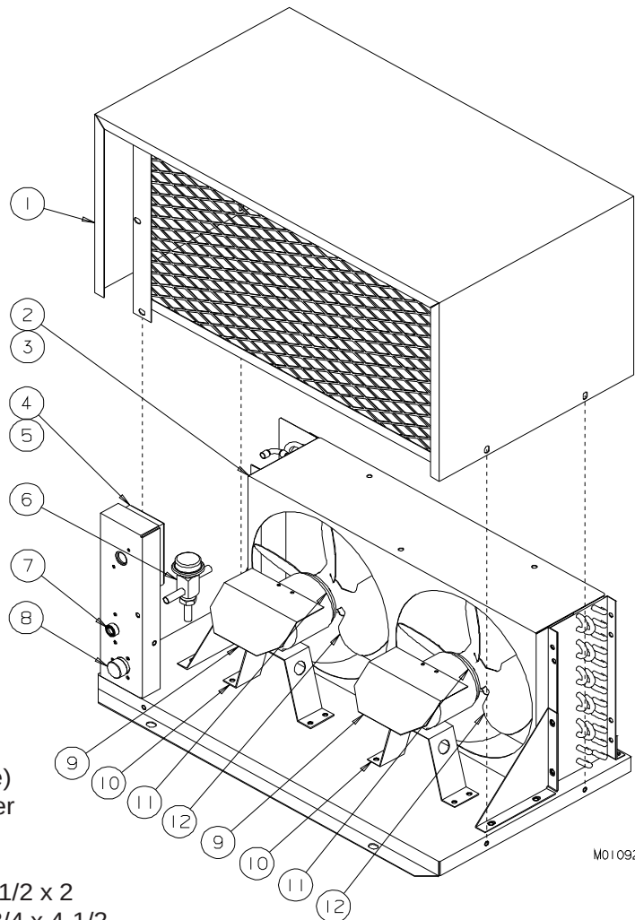
Figure 18 Air Cooled Remote Condenser
