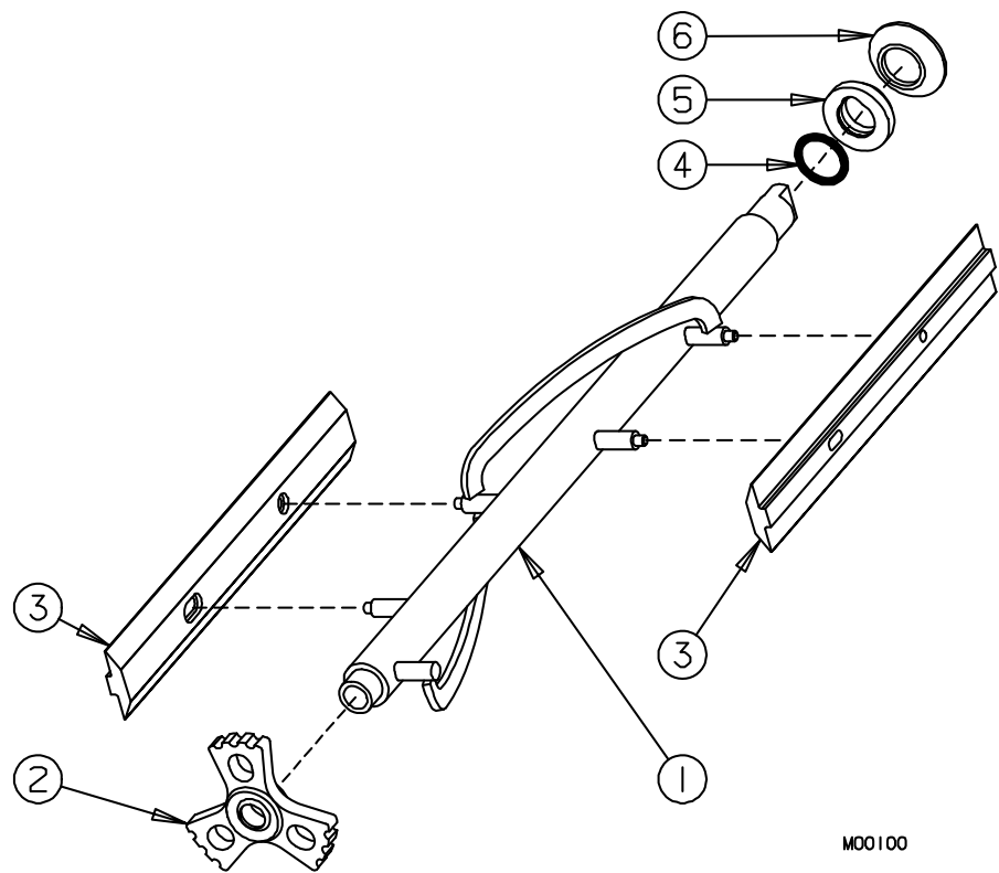
Figure 2 Beater Shaft Assembly
