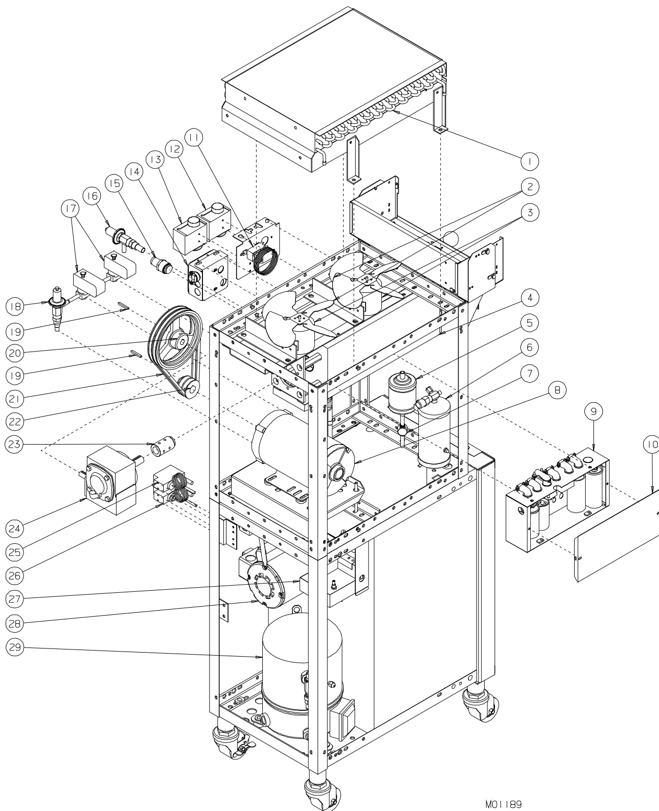
Figure 14 44N-CMT-W Air Cooled Side/Back View (Sheet 1 of 2)
