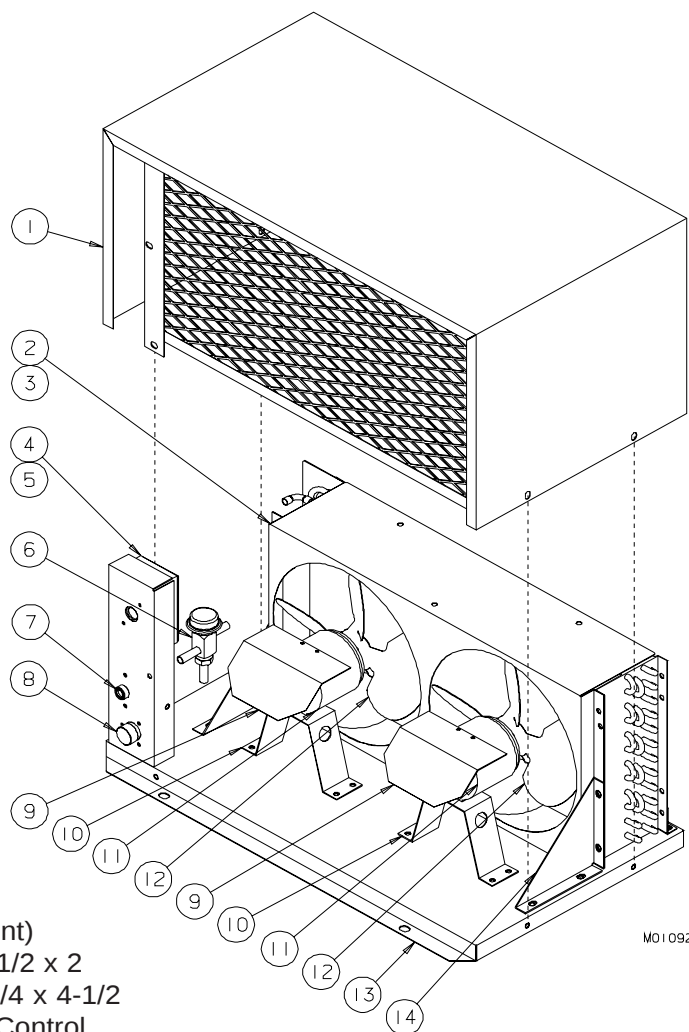
Figure 17 Air Cooled Remote Condenser
