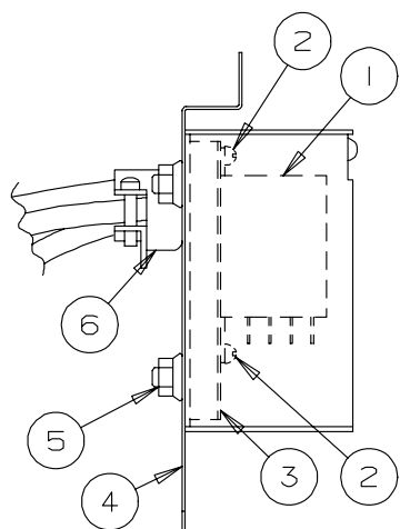
Figure 9 Relay Box — MTS
