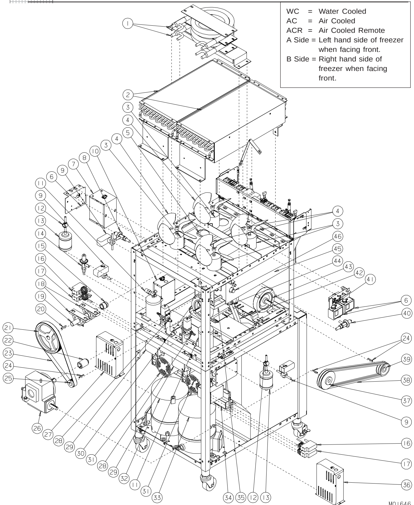
Figure 15 Assembly - Rear View (Sheet 1 of 4)
