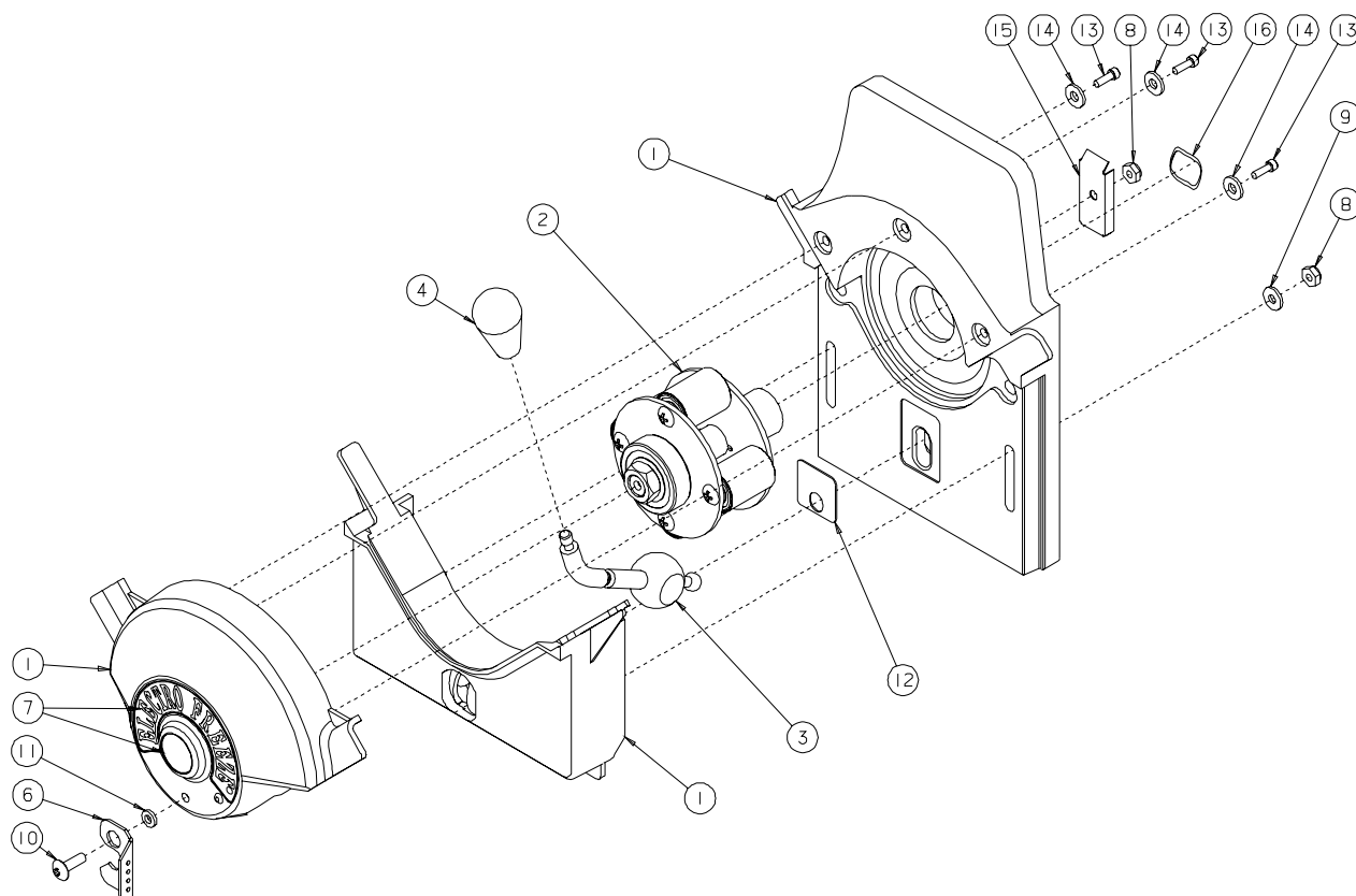
Figure 7 Mix Transfer System (MTS)
