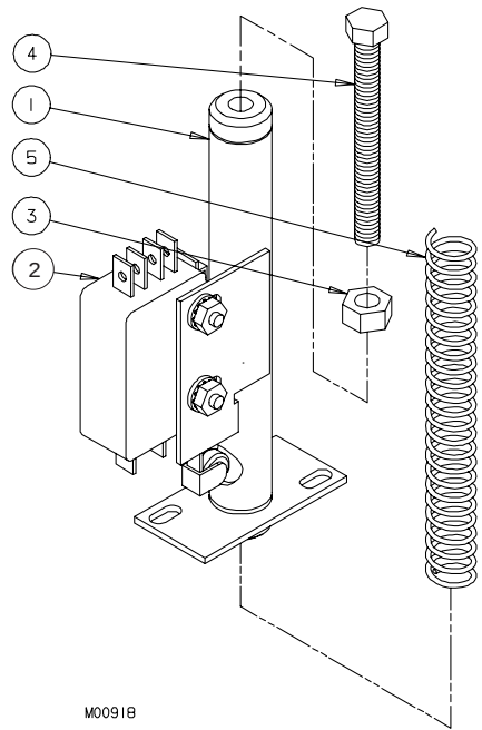
Figure 11 Switch Assembly - Shake
