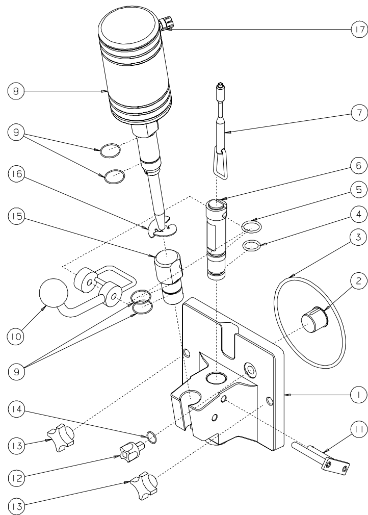
Figure 2 Shake Dispense Head Assembly
