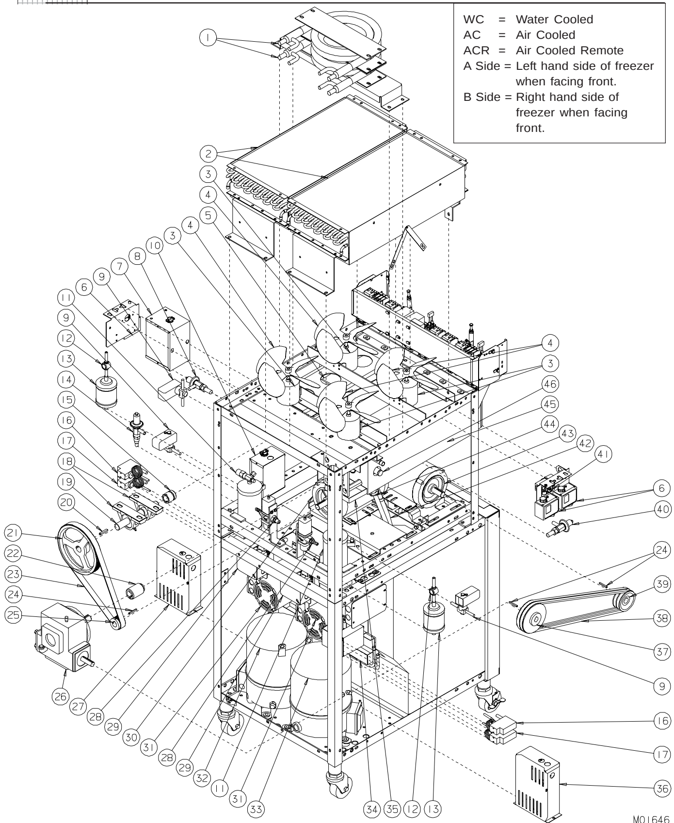
Figure 15 Assembly - Rear View (Sheet 3 of 4)
