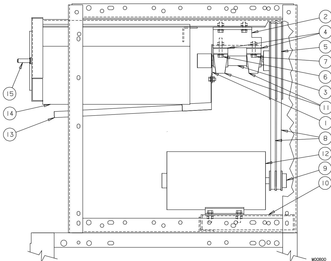
Figure 13 Drive Assembly - Shake
